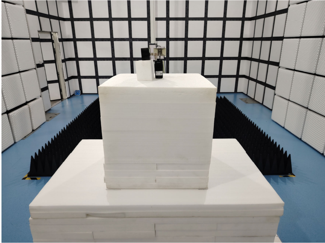
Radiation Emission - Back View (Above 1GHz)
