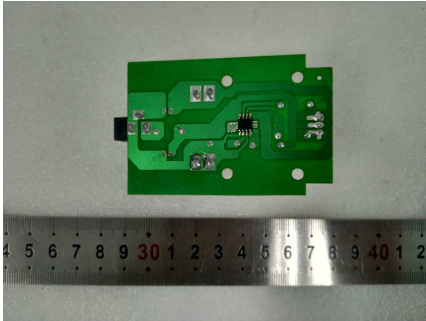
EUT –Base MainBoard Rear View
