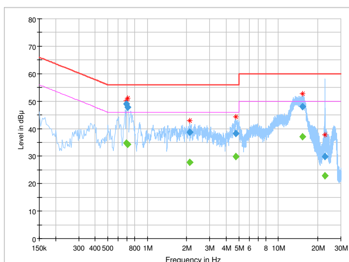
Full Spectrum
