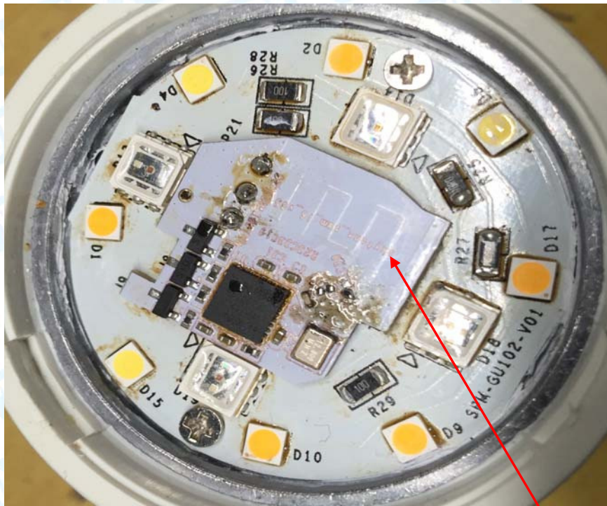
2.4G PCB Antenna
