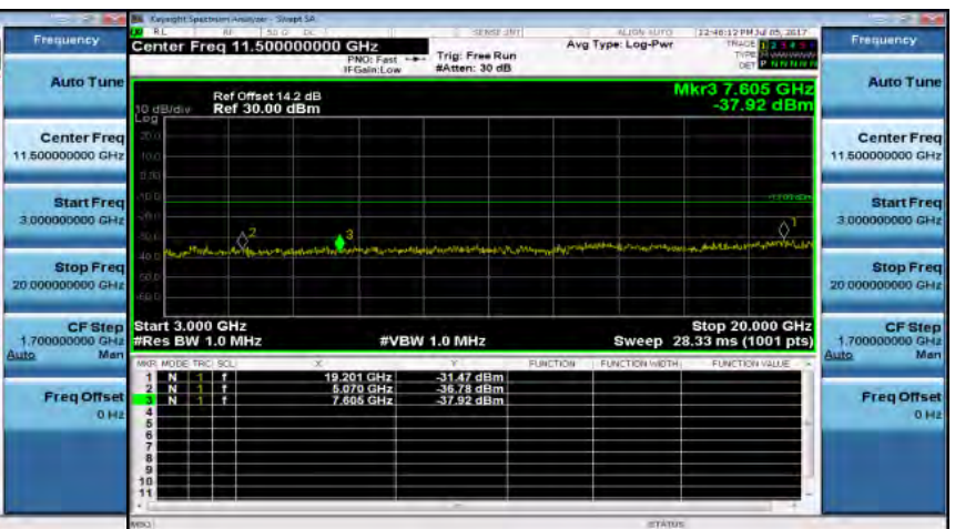
Out of Band Emission High_Band7 20MHz_QPSK 1 0_HighCH21350-2560
