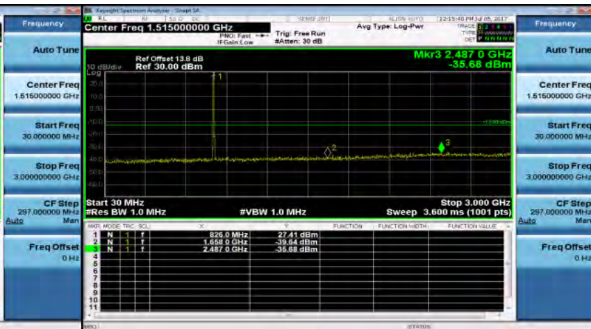
Out of Band Emission Low_Band5 10MHz_QPSK 1 0_MidCH20525-836.5
