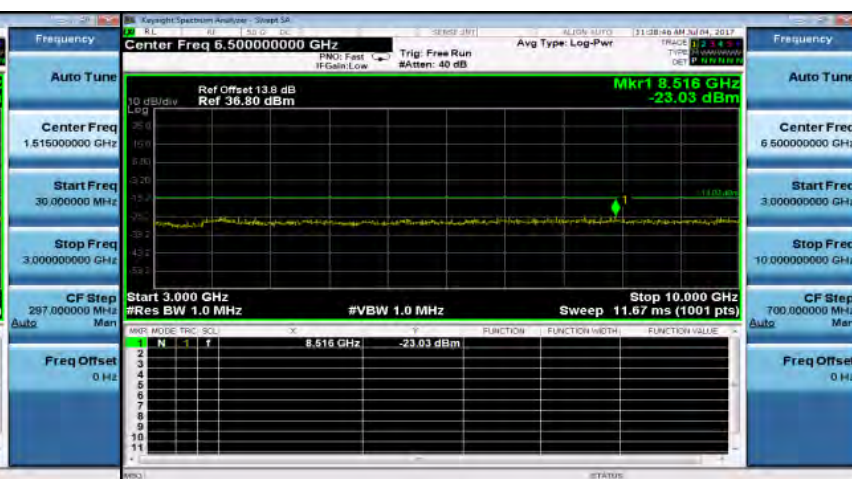
Out of Band Emission High_GSM_850MHz_LowCH128-824.2
