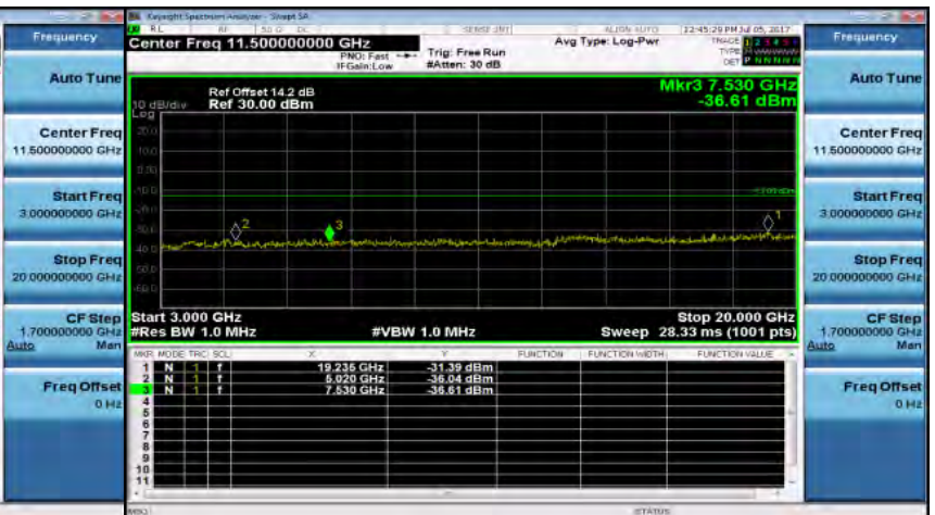
Out of Band Emission High_Band7 20MHz_QPSK 1 0_MidCH21100-2535
