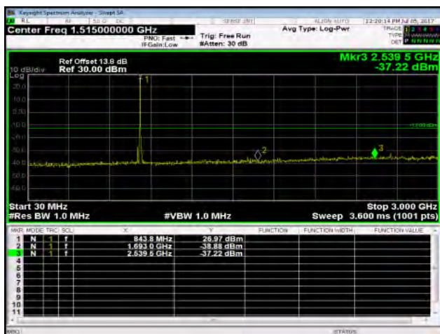
Out of Band Emission Low_Band5 5MHz_QPSK 1 0_HighCH20625-846.5
