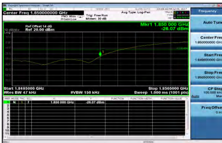
Band Edge_WCDMA_B2_LowCH9262-1852.4
