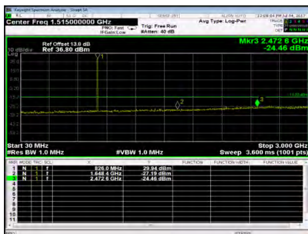
Out of Band Emission Low_EDGE_850MHz_LowCH128-824.2
