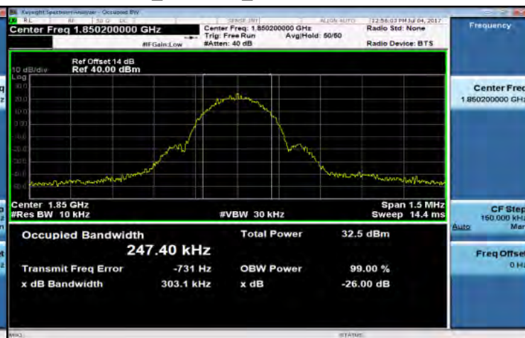
EDGE_1900MHz_LowCH512-1850.2
