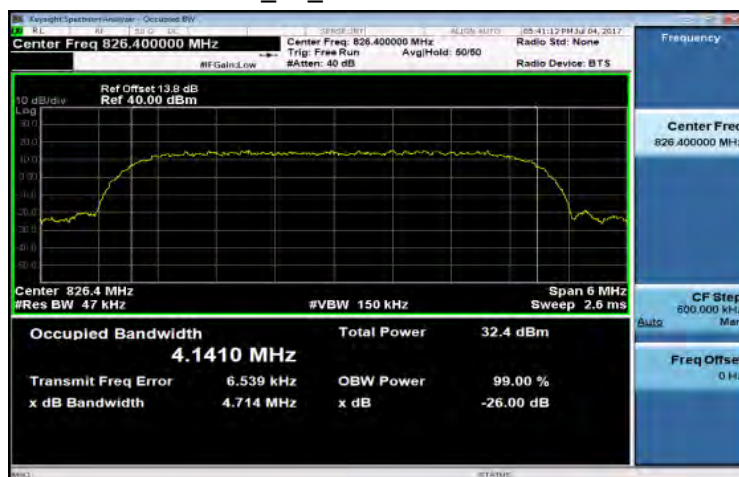
HSDPA_B5_LowCH4132-826.4
