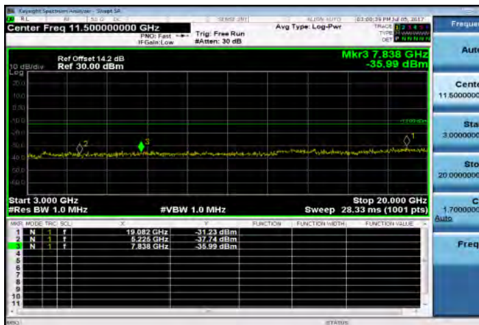
Out of Band Emission High_Band38 15MHz_QPSK 1 0_HighCH38175-2612.5
