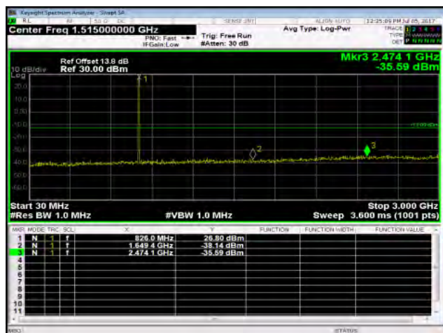
Out of Band Emission Low_Band5 1.4MHz_QPSK 1 0_MidCH20525-836.5
