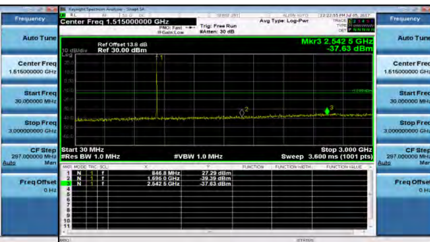
Out of Band Emission Low_Band5 3MHz_QPSK 1 0_HighCH20635-847.5
