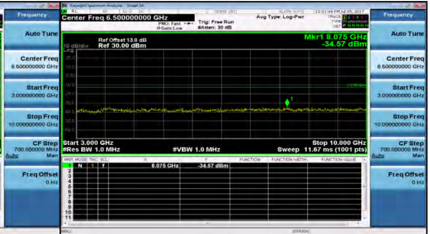
Out of Band Emission High_Band5 3MHz_QPSK 1 0_MidCH20525-836.5
