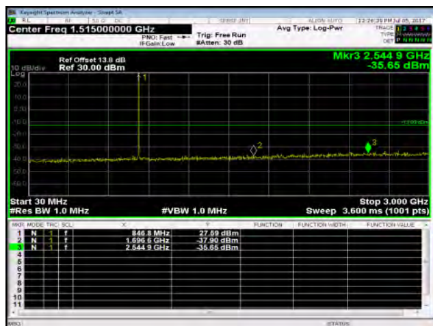
Out of Band Emission Low_Band5 1.4MHz_QPSK 1 0_HighCH20643-848.3
