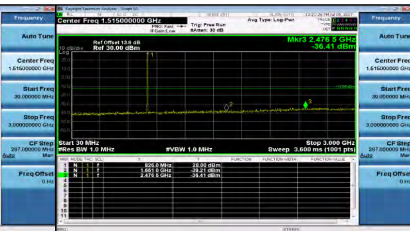
Out of Band Emission Low_Band5 3MHz_QPSK 1 0_MidCH20525-836.5
