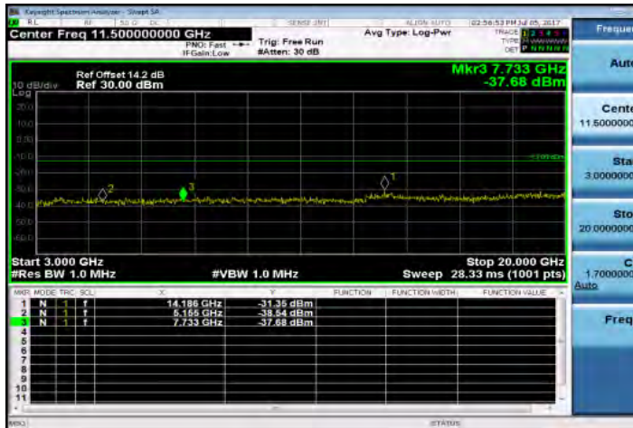
Out of Band Emission High_Band38 15MHz_QPSK 1 0_MidCH38000-2595
