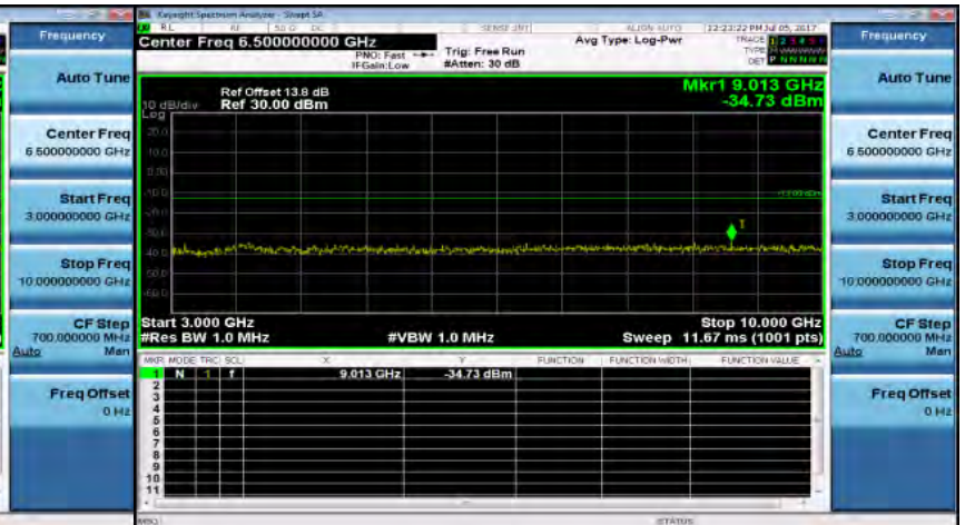
Out of Band Emission High_Band5 3MHz_QPSK 1 0_HighCH20635-847.5
