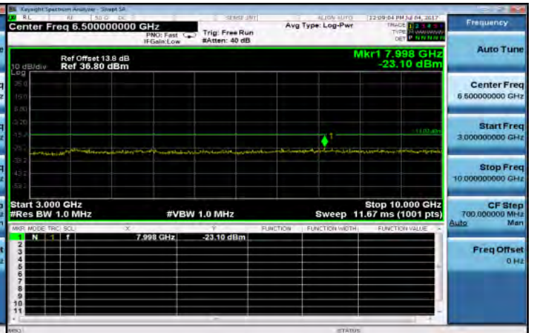
Out of Band Emission High_EDGE_850MHz_LowCH128-824.2
