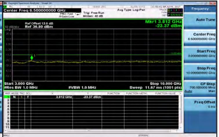
Out of Band Emission High_GPRS_850MHz_HighCH251-848.8
