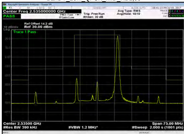
Band 7 20M QPSK MID RB100,0
