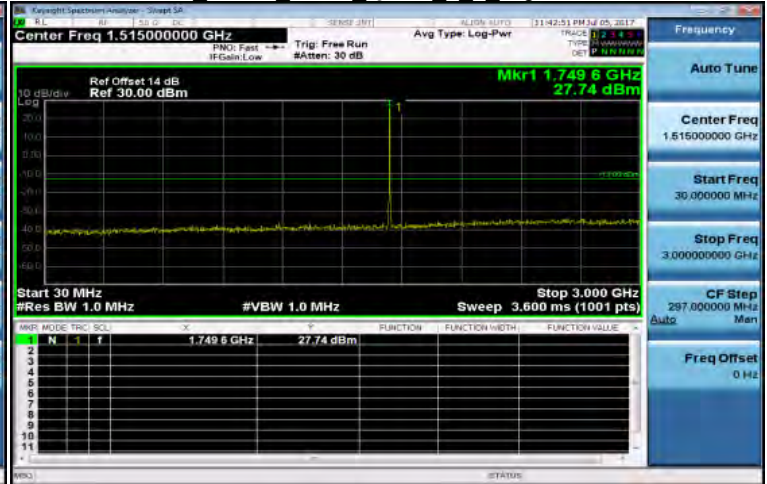
30MHz~3GHz Band4 5MHz QPSK 1 0 HighCH20375-1752.5
