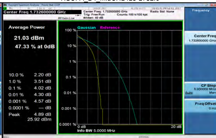
HSUPA B4 MidCH1413-1732.6
