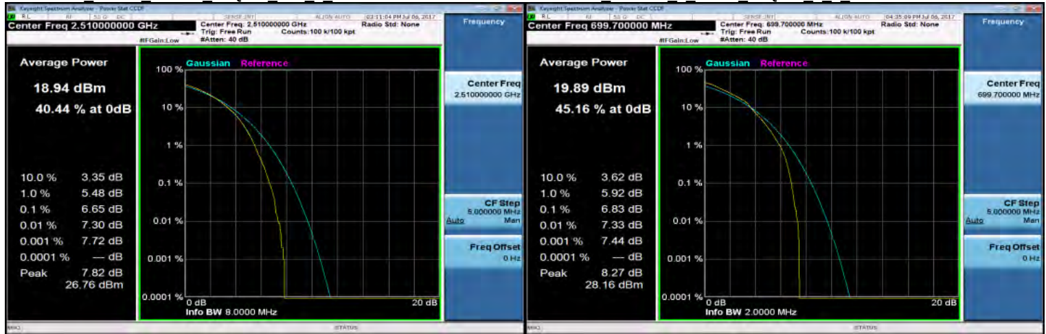
LTE Band7 20MHz 16QAM 100 0 LowCH20850-2510
