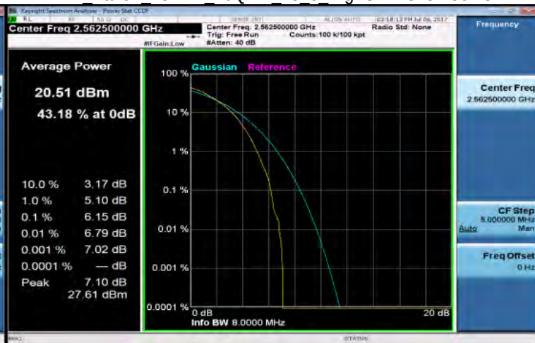
LTE Band7 15MHz 16QAM 75 0 HighCH21375-2562.5
