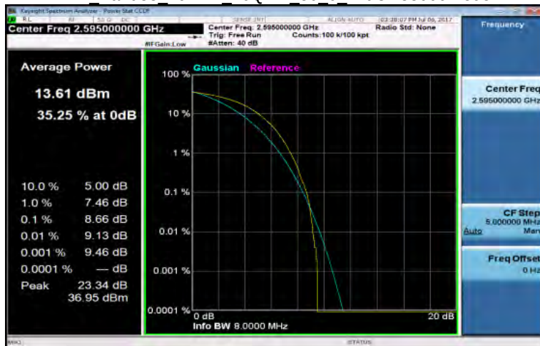
LTE Band38 10MHz 16QAM 50 0 MidCH38000-2595
