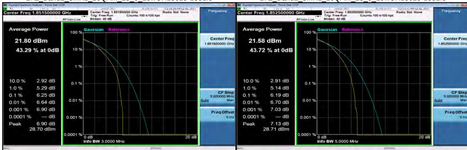
LTE Band2 3MHz 16QAM 15 0 LowCH18615-1851.5
