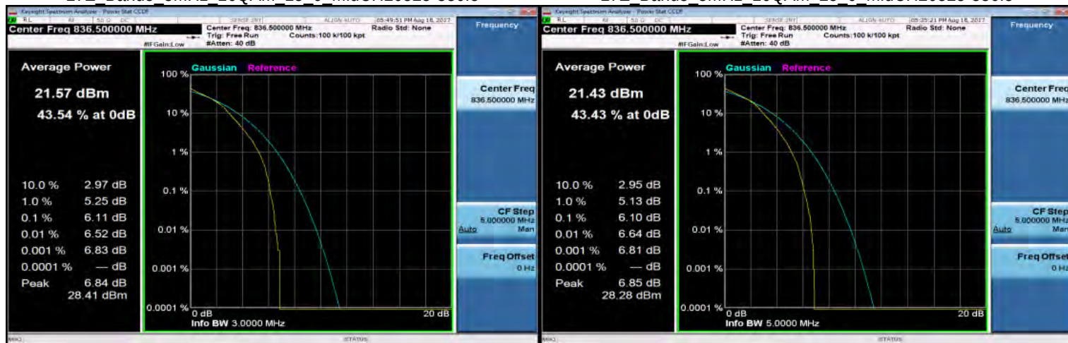
LTE Band5 3MHz 16QAM 15 0 MidCH20525-836.5
