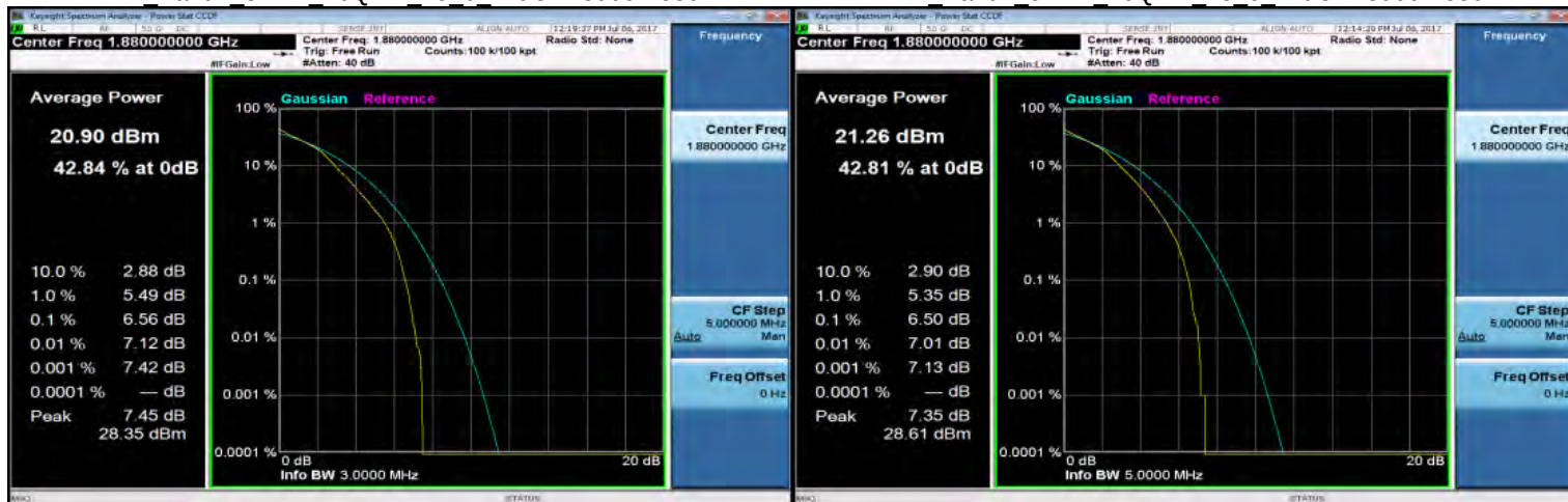
LTE Band2 3MHz 16QAM 15 0 MidCH18900-1880
