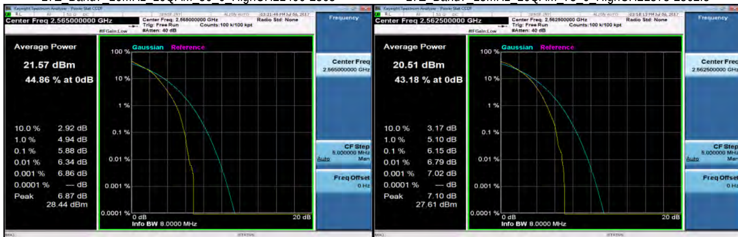
LTE Band7 10MHz 16QAM 50 0 HighCH21400-2565
