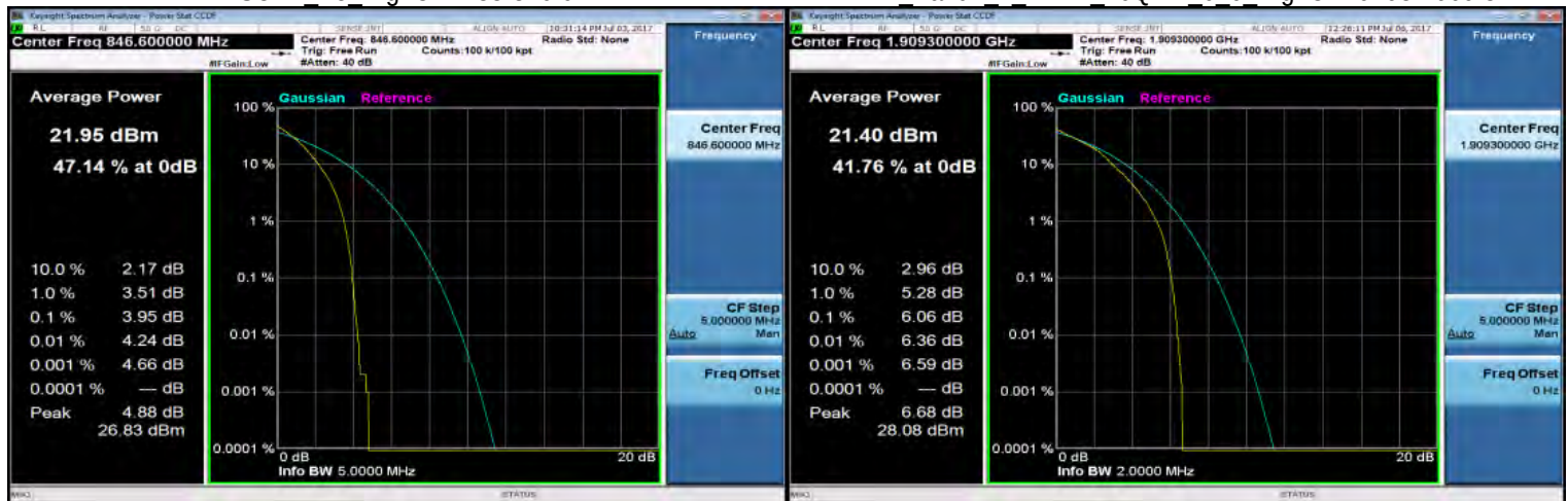
HSUPA B5 HighCH4233-846.6
