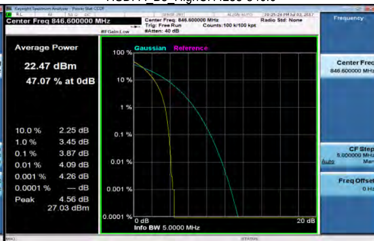
HSDPA B5 HighCH4233-846.6
