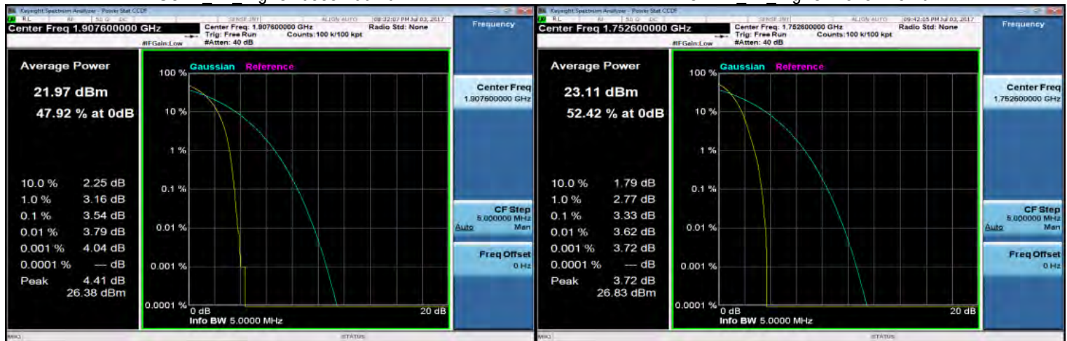
HSUPA B2 HighCH9538-1907.6
