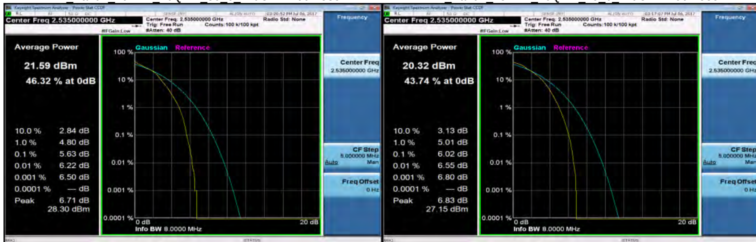
LTE Band7 10MHz 16QAM 50 0 MidCH21100-2535
