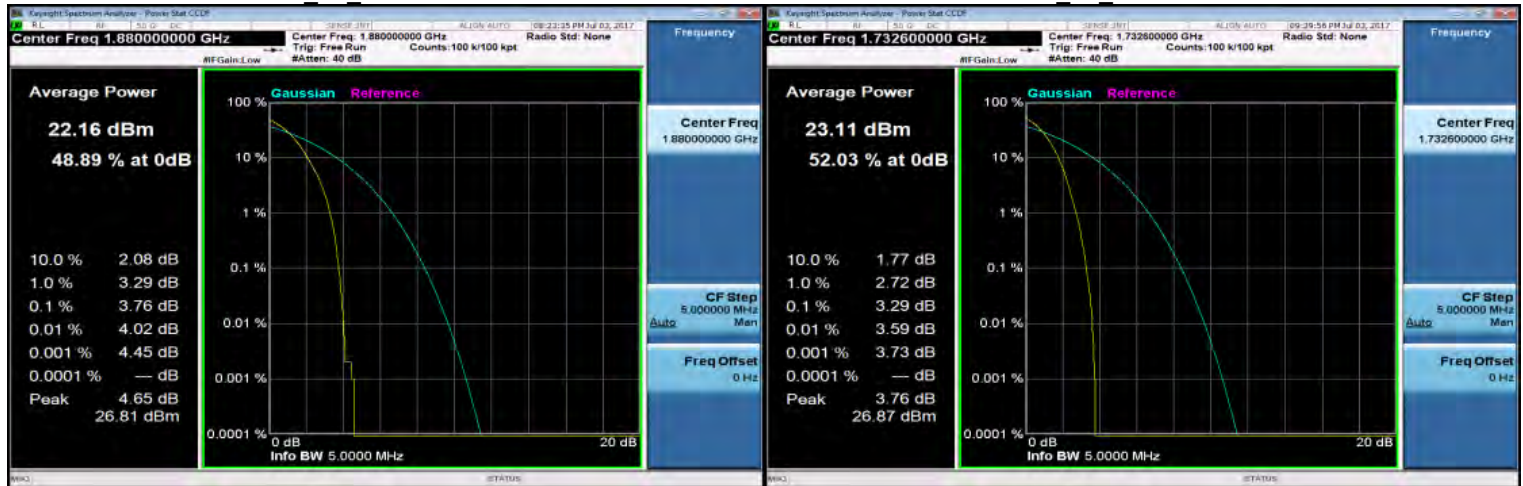
HSUPA B2 MidCH9400-1880
