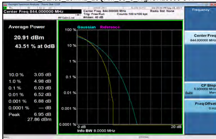
LTE Band5 10MHz 16QAM 50 0 HighCH20600-844
