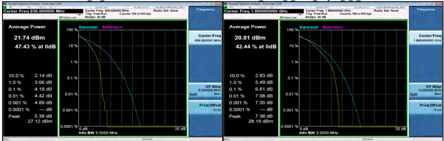
HSUPA B5 MidCH4183-836.6
