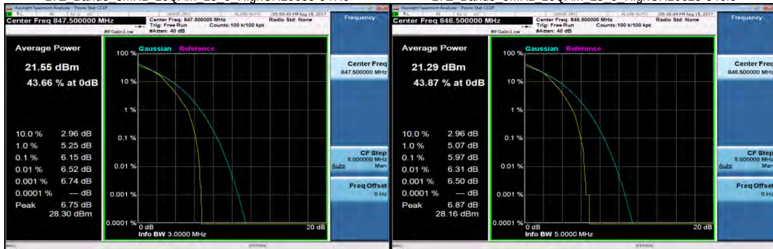
LTE Band5 3MHz 16QAM 15 0 HighCH20635-847.5
