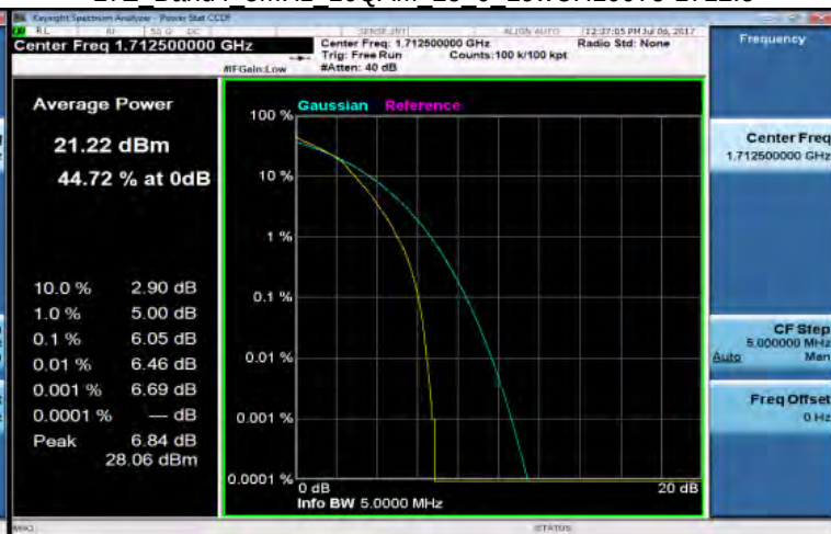
LTE Band4 5MHz 16QAM 25 0 LowCH19975-1712.5
