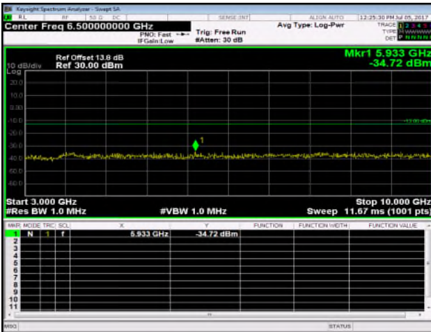
Out of Band Emission High_Band5 1.4MHz_QPSK 1 0_MidCH20525-836.5
