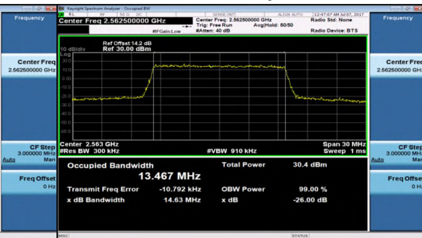
Band7 15MHz_16-QAM 75 0_HighCH21375-2562.5
