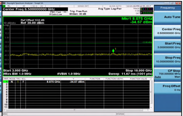
Out of Band Emission High_Band5 3MHz_QPSK 1 0_MidCH20525-836.5
