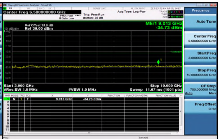
Out of Band Emission High_Band5 3MHz_QPSK 1 0_HighCH20635-847.5
