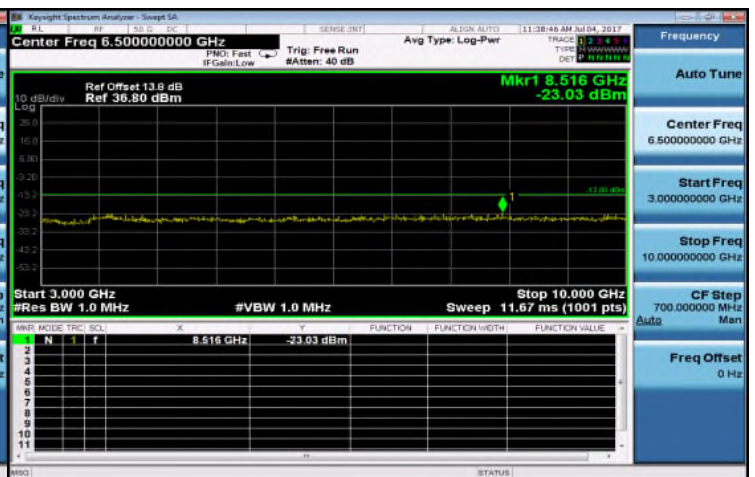
Out of Band Emission High_GSM_850MHz_LowCH128-824.2
