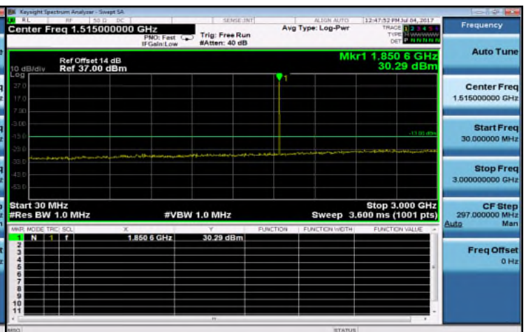
Out of Band Emission Low_GPRS_1900MHz_LowCH512-1850.2
