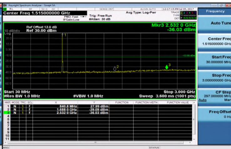
Out of Band Emission Low_Band5 10MHz_QPSK 1 0_HighCH20600-844
