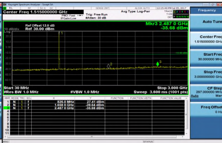
Out of Band Emission Low_Band5 10MHz_QPSK 1 0_MidCH20525-836.5
