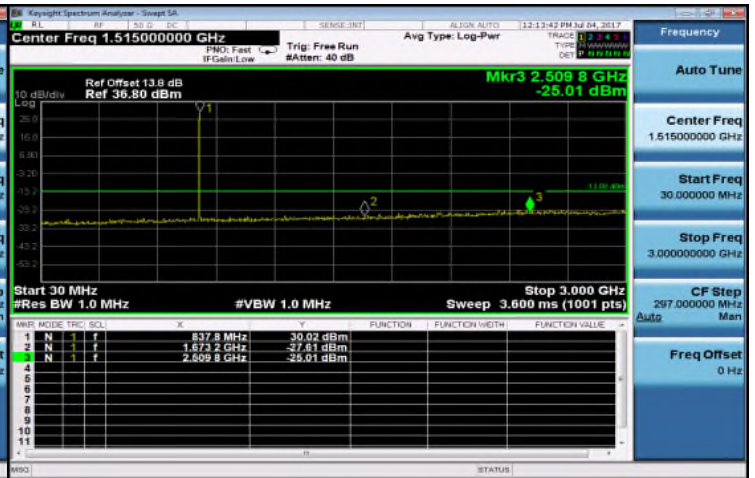
Out of Band Emission Low_EDGE_850MHz_HighCH251-848.8
