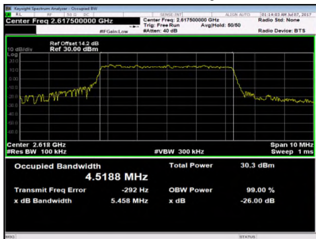
Band38 5MHz_QPSK 25 0_HighCH38225-2617.5
