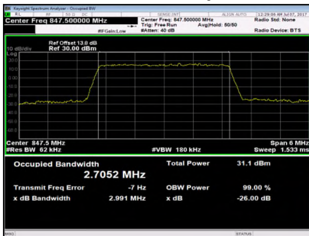
Band5 3MHz_QPSK 15 0_HighCH20635-847.5
