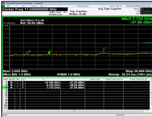
Out of Band Emission High_Band38 15MHz_QPSK 1 0_MidCH38000-2595
