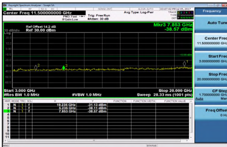
Out of Band Emission High_Band38 5MHz_QPSK 1 0_HighCH38225-2617.5
