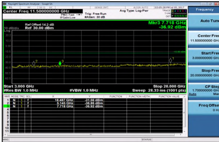
Out of Band Emission High_Band38 5MHz_QPSK 1 0_MidCH38000-2595
