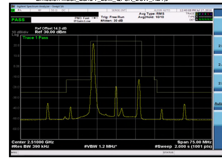
Emission Mask_Band 7_20M_QPSK_LOW_RB1,0
