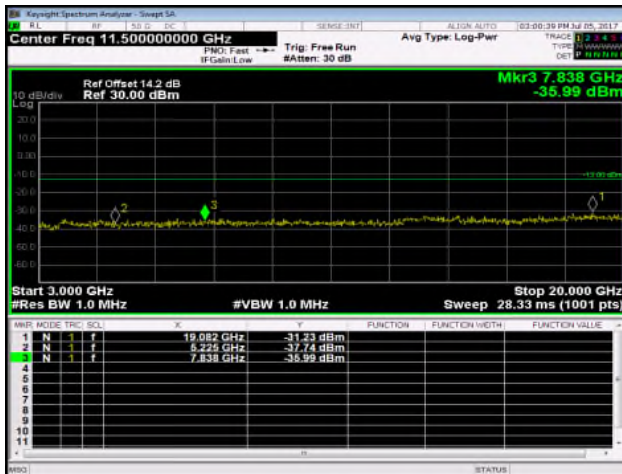
Out of Band Emission High_Band38 15MHz_QPSK 1 0_HighCH38175-2612.5
