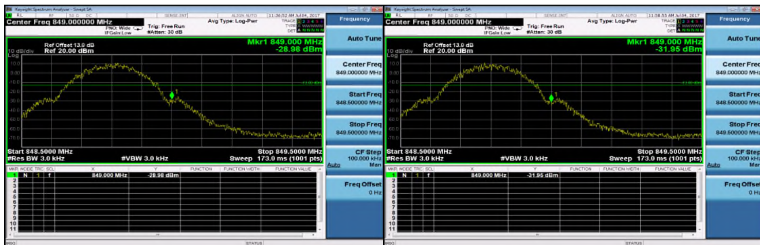
Band Edge_GSM_850MHz_HighCH251-848.8
