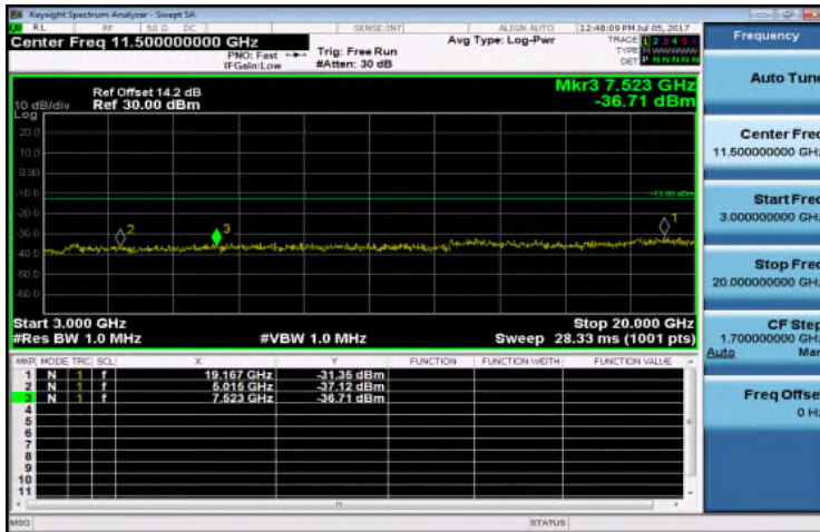
Out of Band Emission High_Band7 15MHz_QPSK 1 0_MidCH20175-1732.5
