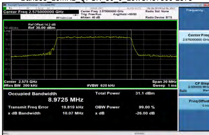
Band38 10MHz QPSK 50 0 LowCH37800-2575
