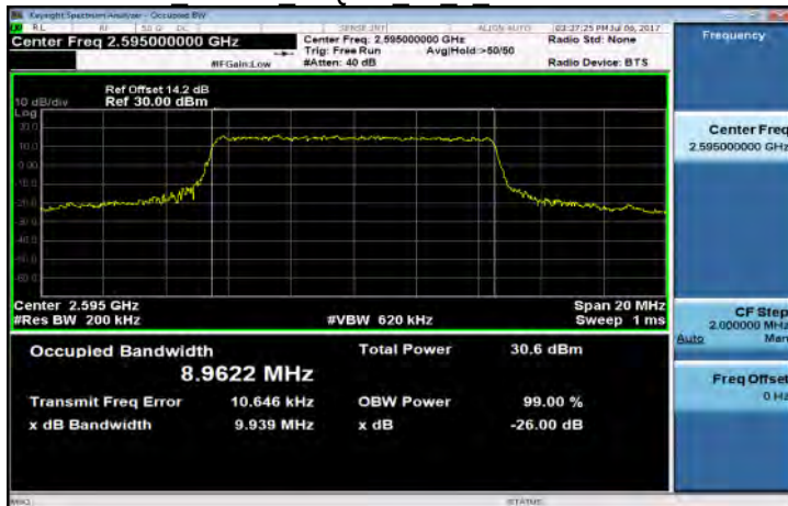
Band38 10MHz 16QAM 50 0 MidCH38000-2595
