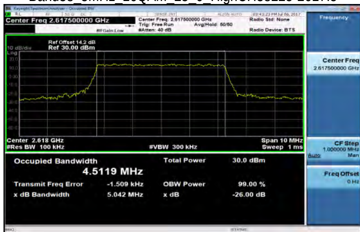
Band38 5MHz 16QAM 25 0 HighCH38225-2617.5
