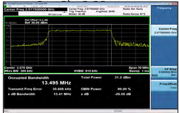
Band38 15MHz QPSK 75 0 LowCH37825-2577.5
