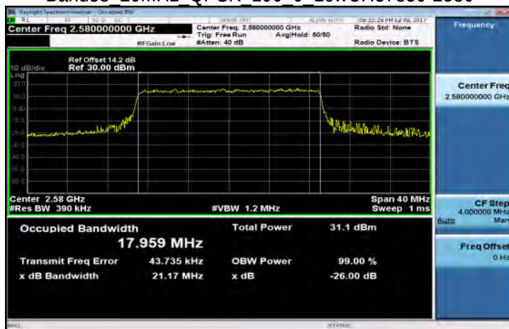
Band38 20MHz QPSK 100 0 LowCH37850-2580
