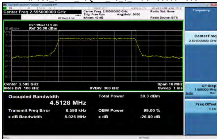
Band38 5MHz 16QAM 25 0 MidCH38000-2595
