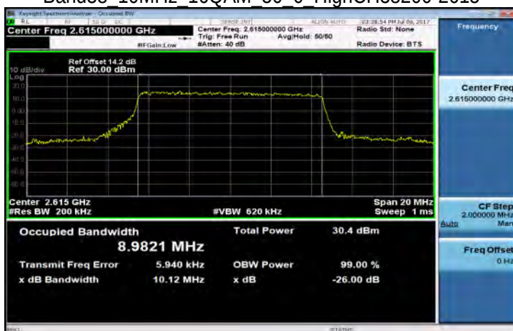
Band38 10MHz 16QAM 50 0 HighCH38200-2615
