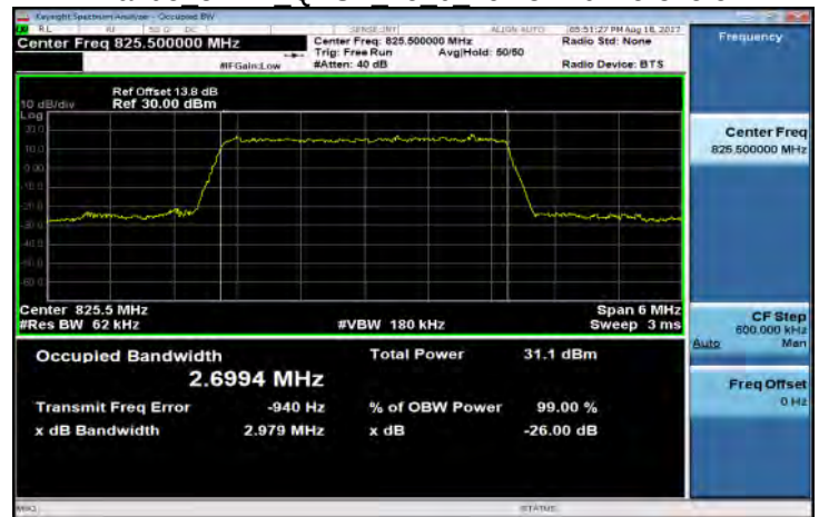
Band5 3MHz QPSK 15 0 LowCH20415-825.5
