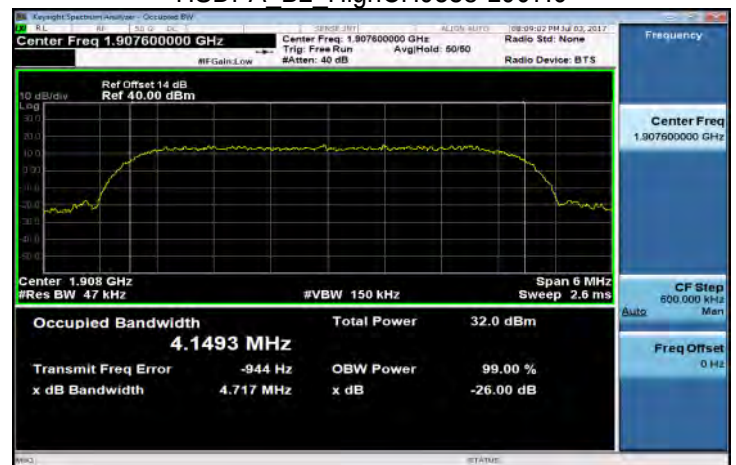
HSDPA B2 HighCH9538-1907.6
