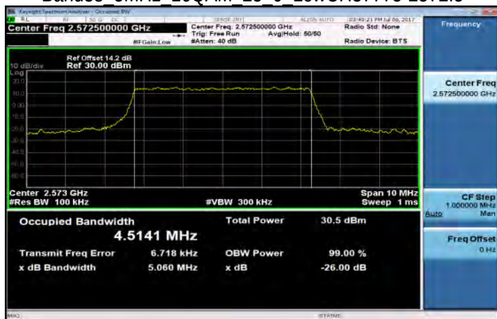
Band38 5MHz 16QAM 25 0 LowCH37775-2572.5
