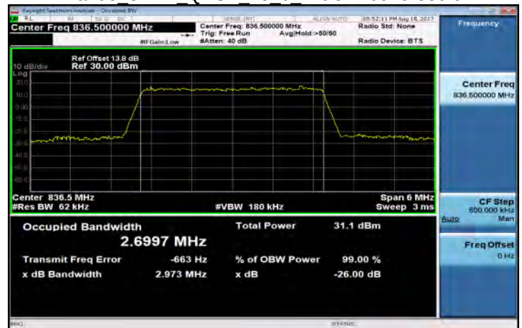
Band5 3MHz QPSK 15 0 MidCH20525-836.5
