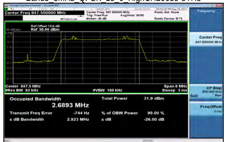
Band5 3MHz QPSK 15 0 HighCH20635-847.5
