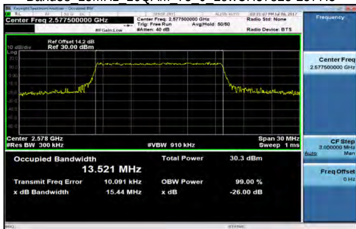
Band38 15MHz 16QAM 75 0 LowCH37825-2577.5
