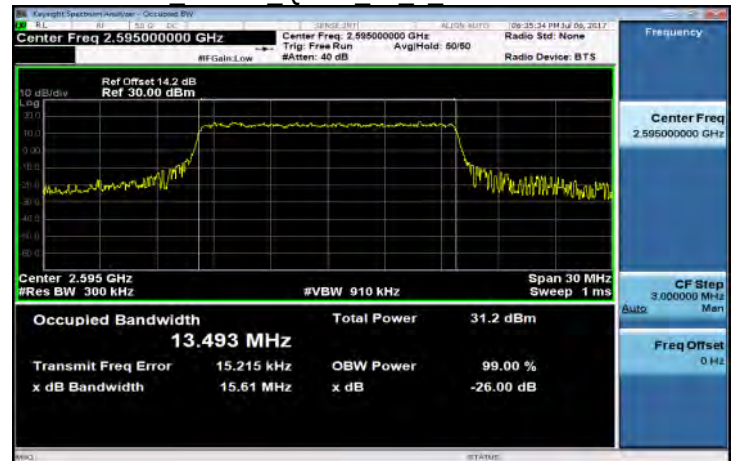
Band38 15MHz QPSK 75 0 MidCH38000-2595
