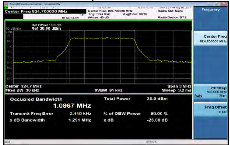
Band5 1 4MHz QPSK 6 0 LowCH20407-824.7
