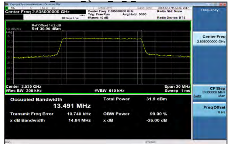
Band7 15MHz QPSK 75 0 MidCH21100-2535
