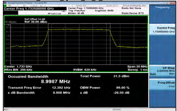
Band4 10MHz QPSK 50 0 MidCH20175-1732.5
