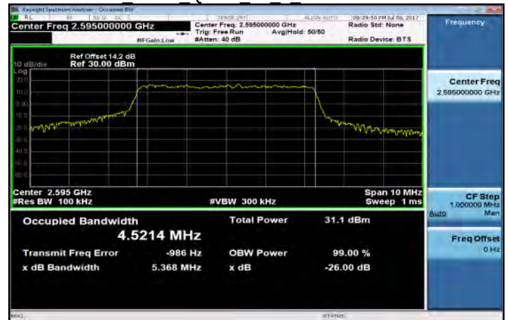
Band38 5MHz QPSK 25 0 MidCH38000-2595
