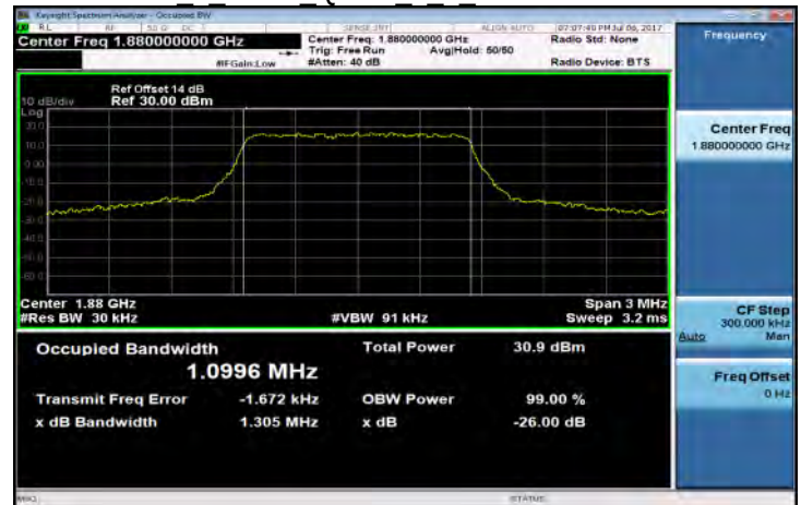
Band2 1 4MHz QPSK 6 0 MidCH18900-1880
