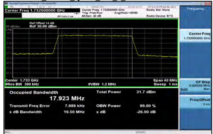
Band4 20MHz QPSK 100 0 MidCH20175-1732.5
