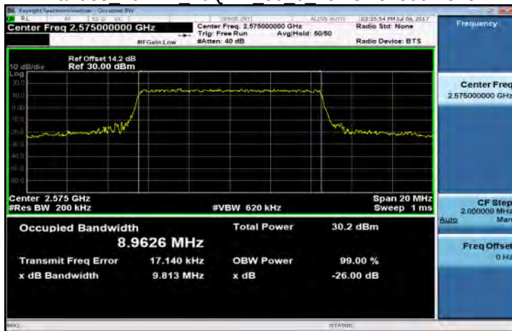
Band38 10MHz 16QAM 50 0 LowCH37800-2575
