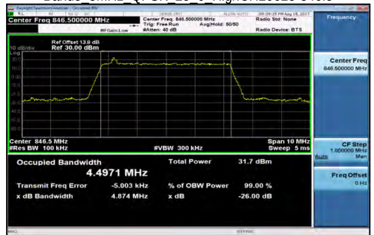
Band5 5MHz QPSK 25 0 HighCH20625-846.5
