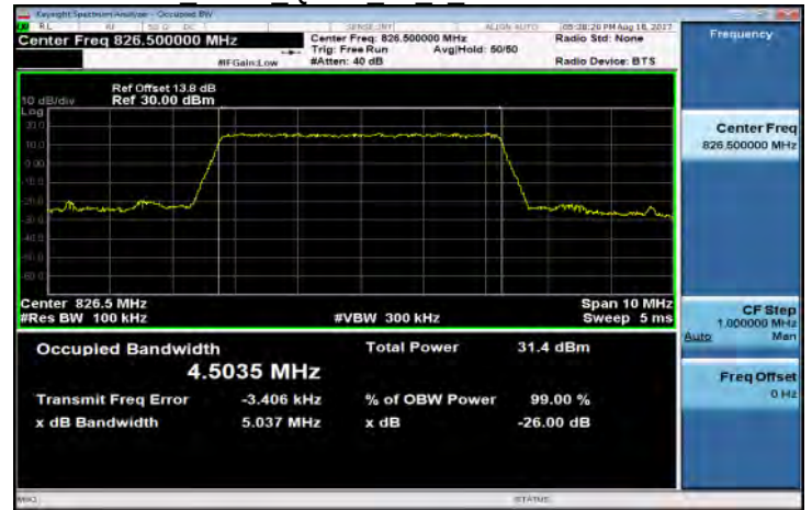
Band5 5MHz QPSK 25 0 LowCH20425-826.5
