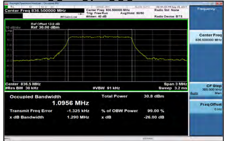
Band5 1 4MHz QPSK 6 0 MidCH20525-836.5
