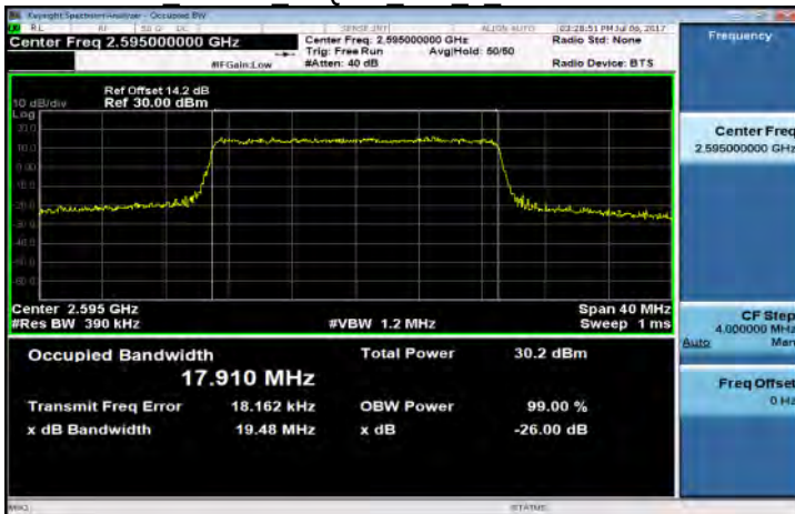
Band38 20MHz 16QAM 100 0 MidCH38000-2595
