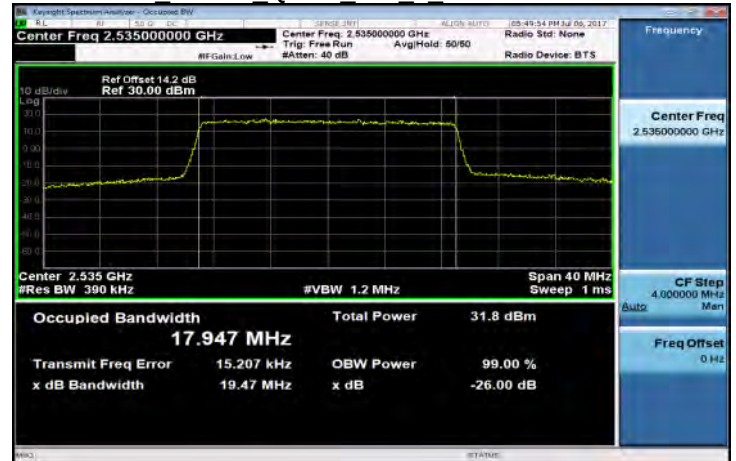
Band7 20MHz QPSK 100 0 MidCH21100-2535
