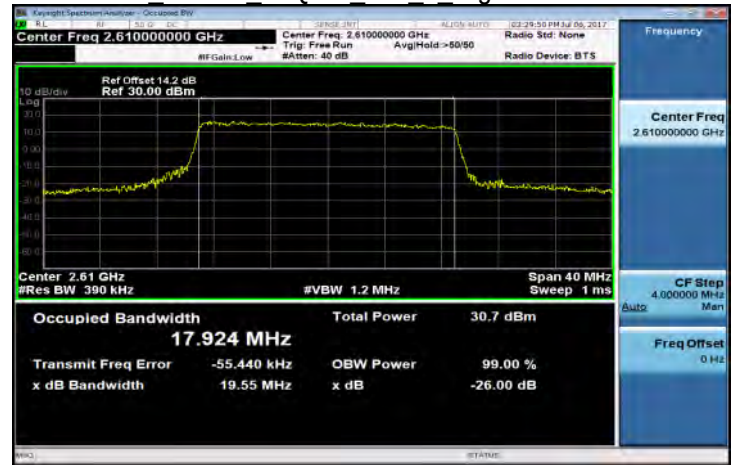
Band38 20MHz 16QAM 100 0 HighCH38150-2610
