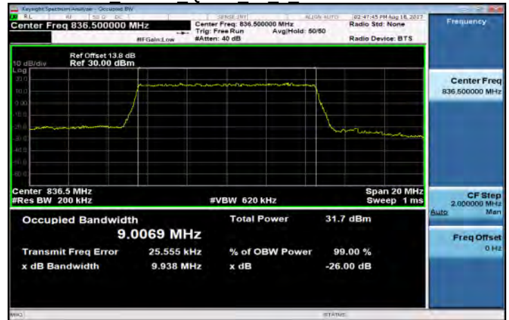
Band5 10MHz QPSK 50 0 MidCH20525-836.5
