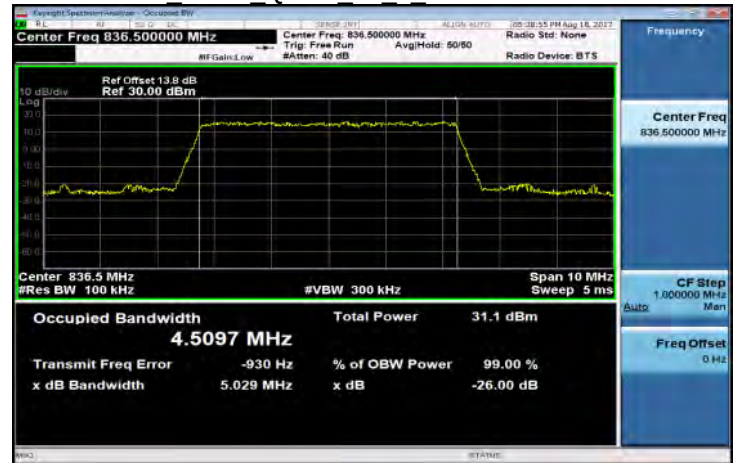
Band5 5MHz QPSK 25 0 MidCH20525-836.5
