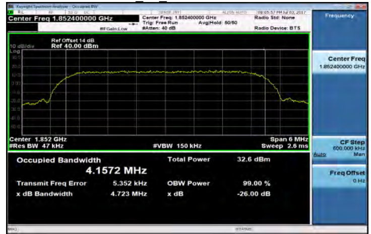
HSDPA B2 LowCH9262-1852.4
