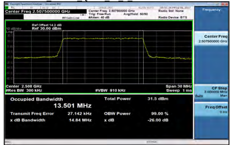
Band7 15MHz QPSK 75 0 LowCH20825-2507.5
