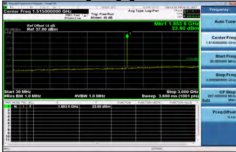
30MHz~3GHz HSUPA B2 LowCH9262-1852.4
