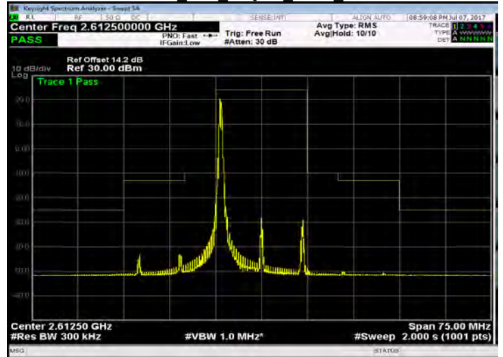
Band 38 15M 16QAM HIGH RB1,74
