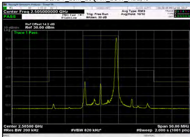
Band 7 10M 16QAM LOW RB5,0
