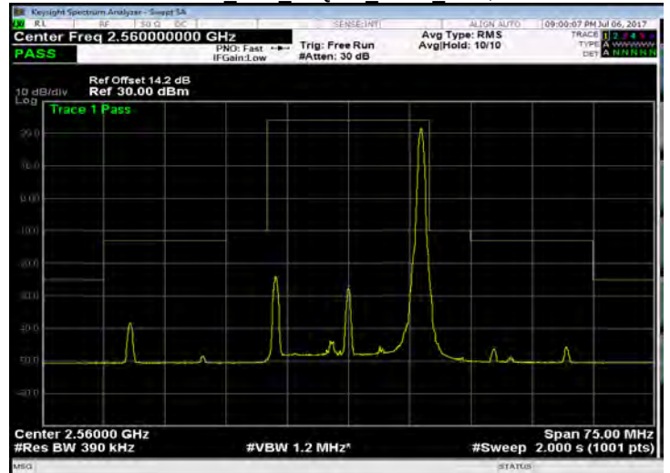
Band 7 20M 16QAM HIGH RB100,0
