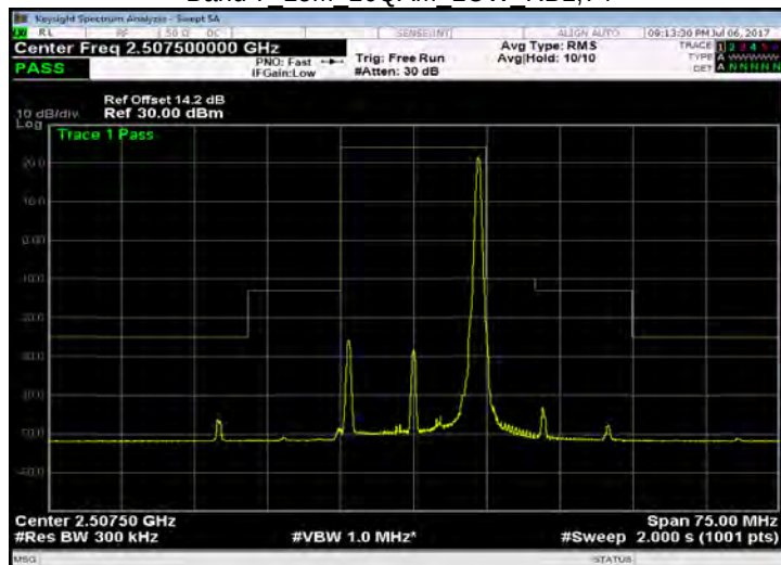
Band 7 15M 16QAM LOW RB75,0
