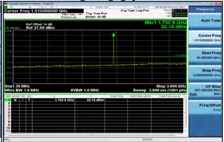
30MHz~3GHz HSDPA B4 HighCH1513-1752.6
