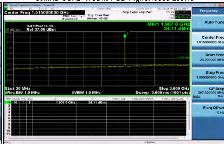
30MHz~3GHz WCDMA B2 HighCH9538-1907.6
