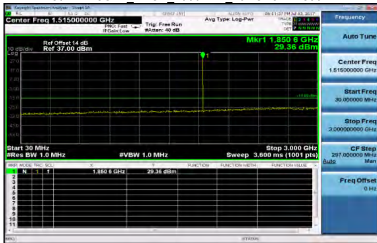
30MHz~3GHz EDGE 1900MHz LowCH512-1850.2
