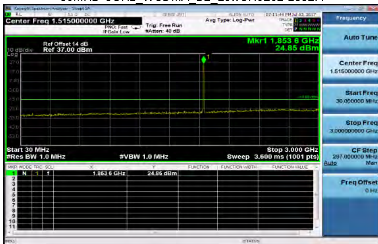
30MHz~3GHz WCDMA B2 LowCH9262-1852.4
