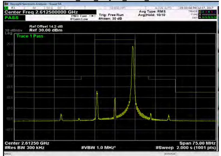
Band 38 15M 16QAM HIGH RB75,0
