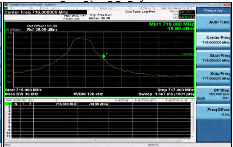
Band12 3MHz QPSK 1 14 HighCH23165-714.5
