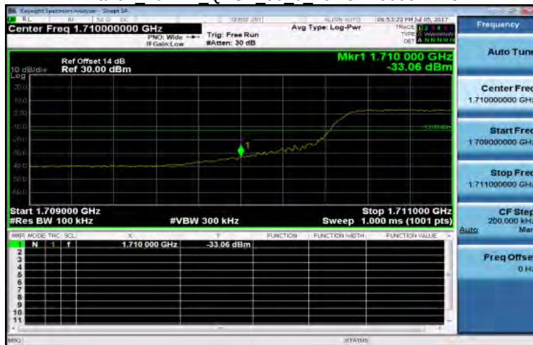
Band4 10MHz QPSK 50 0 LowCH20000-1715
