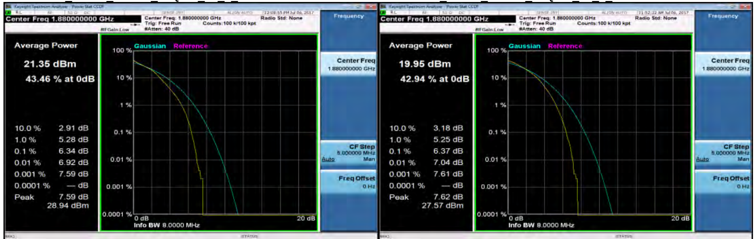
LTE Band2 10MHz 16QAM 50 0 MidCH18900-1880
