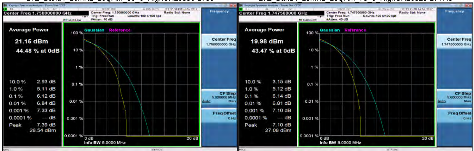
LTE Band4 10MHz 16QAM 50 0 HighCH20350-1750
