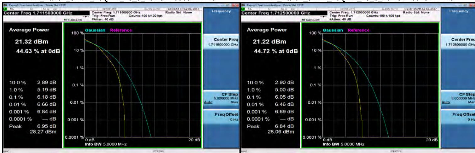
LTE Band4 3MHz 16QAM 15 0 LowCH19965-1711.5
