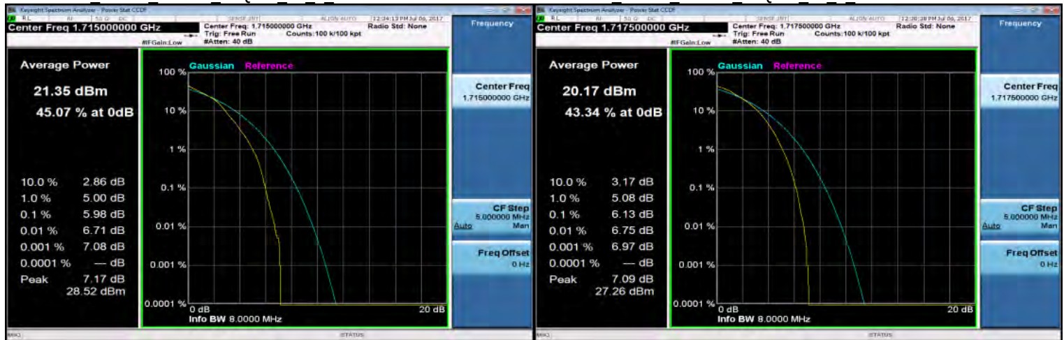
LTE Band4 10MHz 16QAM 50 0 LowCH20000-1715
