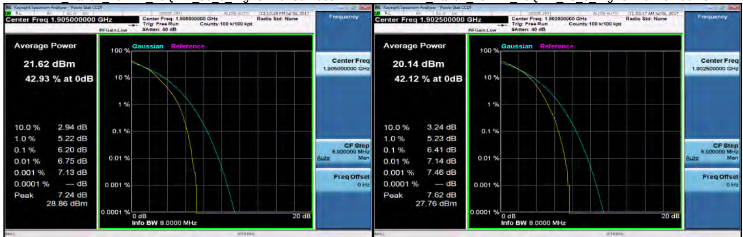
LTE Band2 10MHz 16QAM 50 0 HighCH19150-1905
