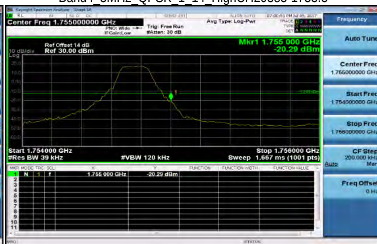
Band4 3MHz QPSK 1 14 HighCH20385-1753.5
