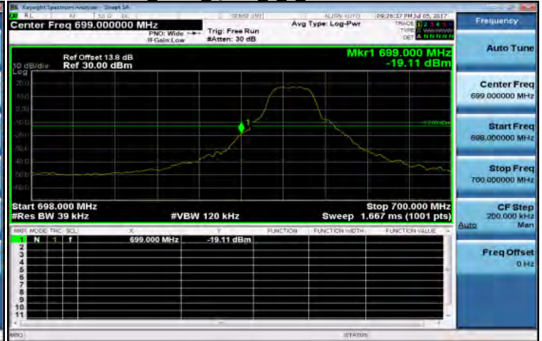
Band12 3MHz QPSK 1 0 LowCH23025-700.5
