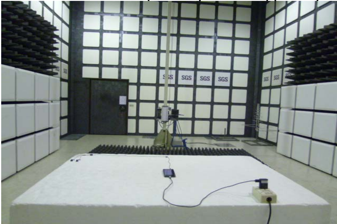
Radiated Emission Set up Photos (Above 1GHz) (E2 Plan)
