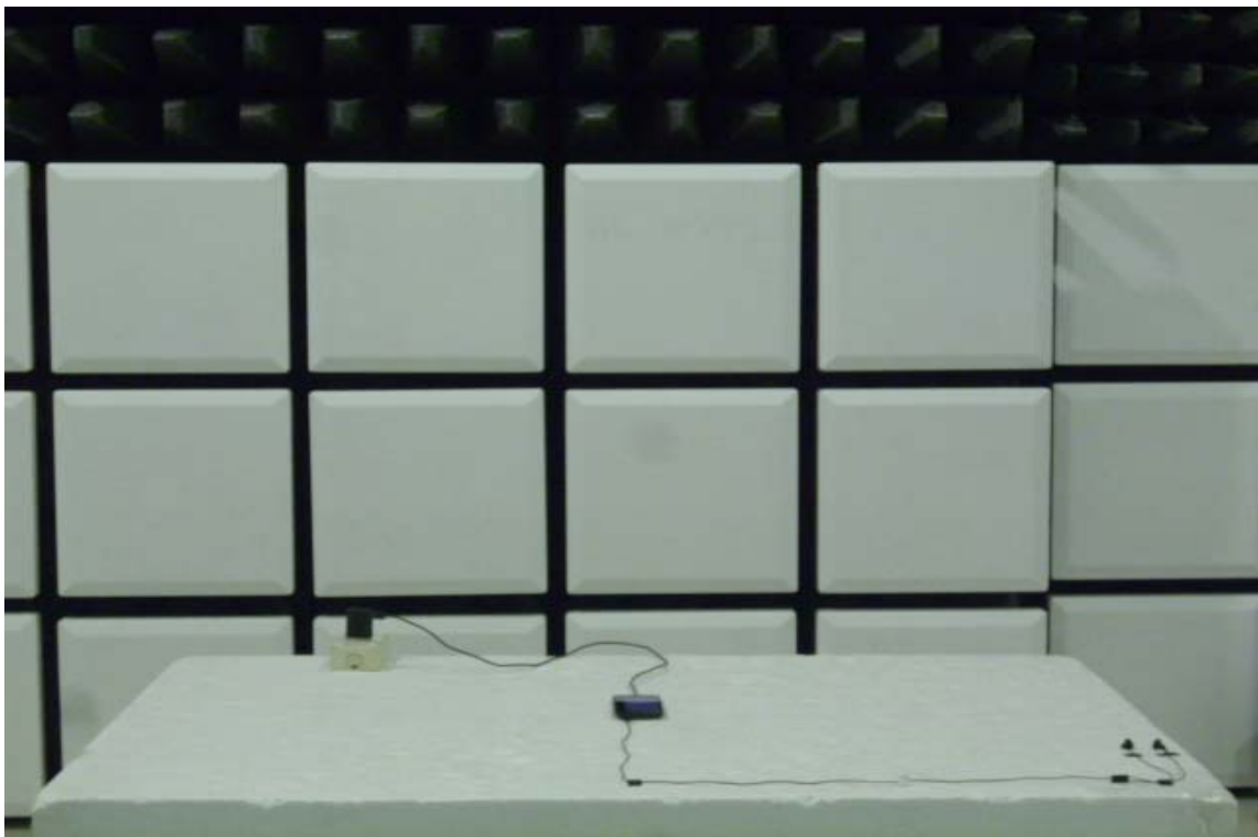
Radiated Emission Set up Photos (Below 1GHz)(H Plan)
