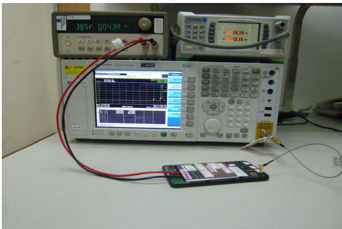
BLE Conducted Setup Photo (Measurement at Antenna Port)
