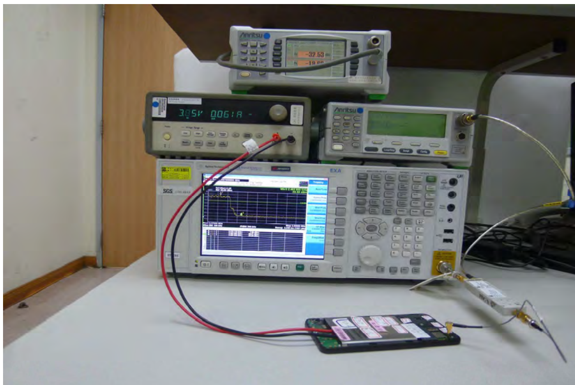
BT Conducted Setup Photo (Measurement at Antenna Port)
