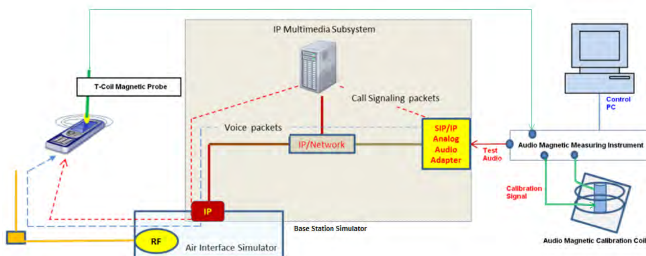
Fig-3.9 Testing Setup for VoLTE, VoWiFi and OTT VoIP
