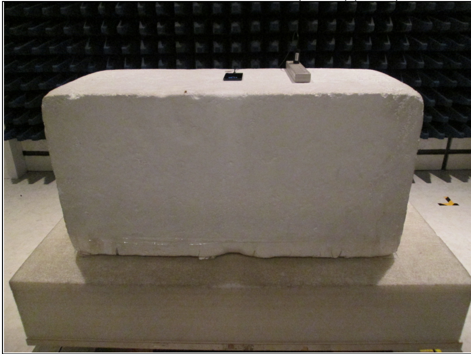
Radiated Emission Test above 1GHz (WWAN) (X-Axis)
