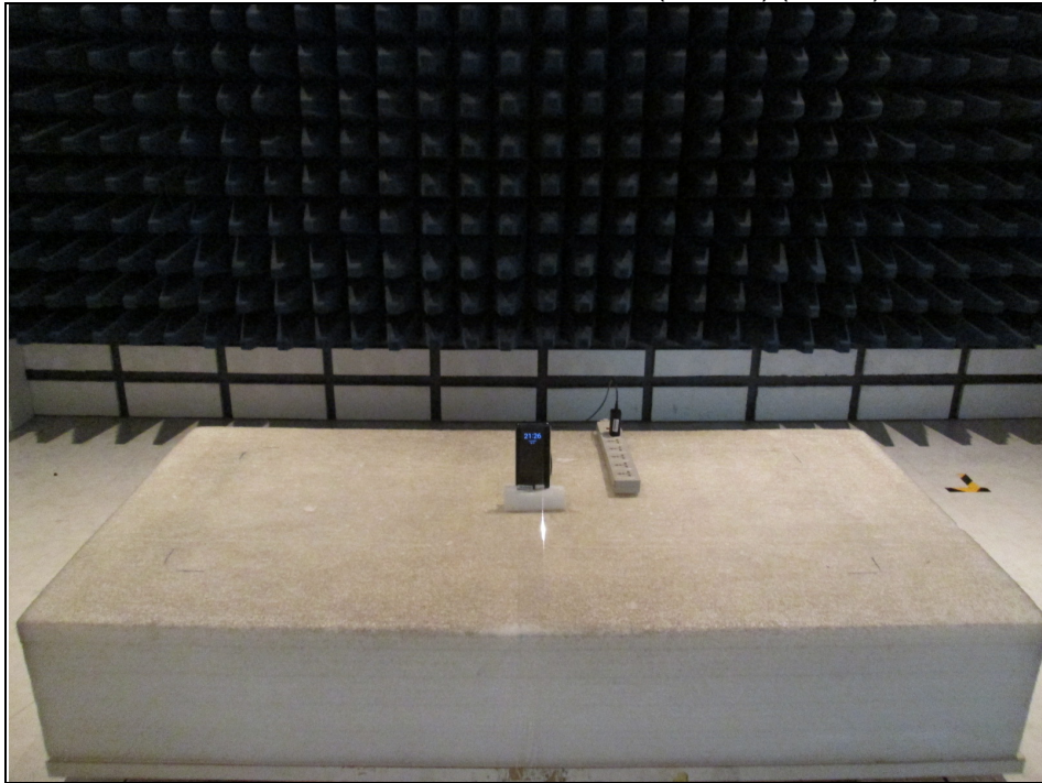
Radiated Emission Test below 1GHz (WWAN) (Z-Axis)
