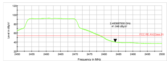
802.11g-Channel 11 Average
