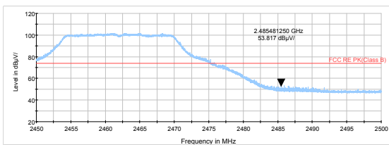
802.11g-Channel 11 Peak
