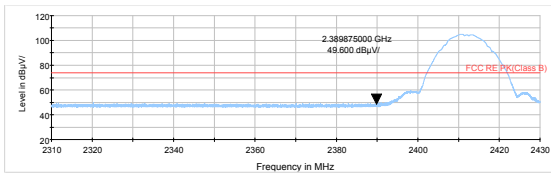
802.11b-Channel 1 Peak
