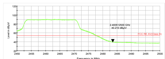
802.11n HT20 -Channel 11 Average
