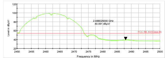
802.11b-Channel 11 Average
