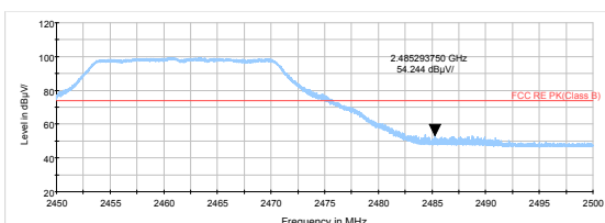
802.11n HT20 -Channel 11 Peak
