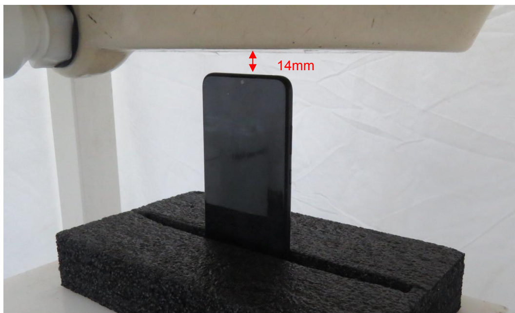
Picture 13: Top Side, the distance from handset to the bottom of the Phantom is 14mm
