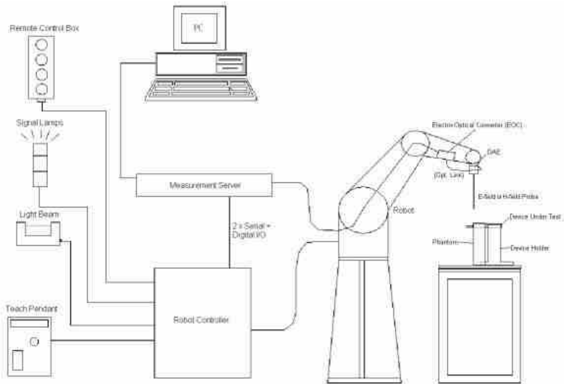
Fig 5.1 System Configurations
