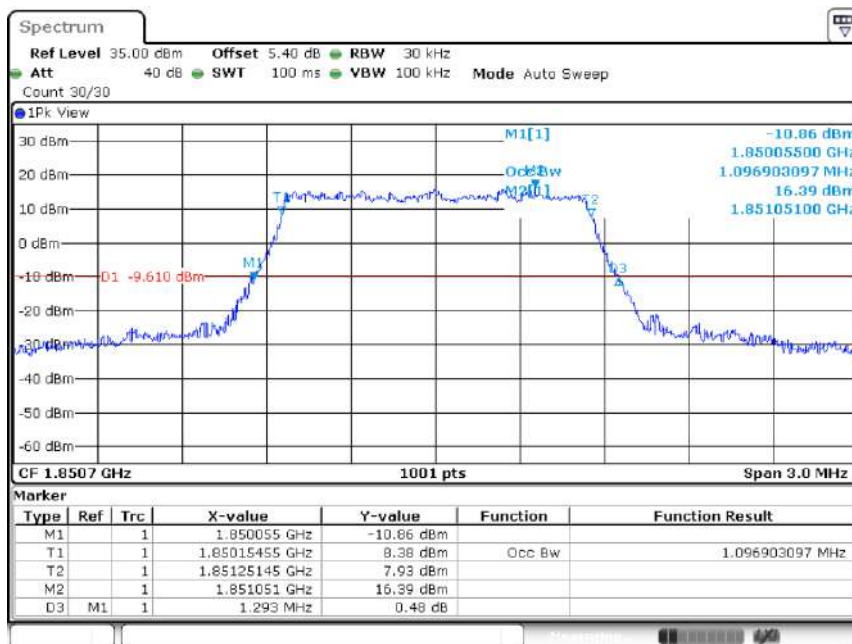
Band2-1.4MHz-64QAM-18607-6RB#0-1.097
