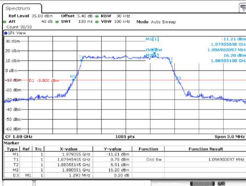
Band2-1.4MHz-64OAM-18900-6RB#0-1.097
