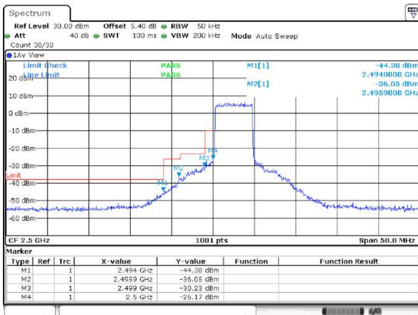
Band7-5MHz-QPSK-20775-25RB#0
