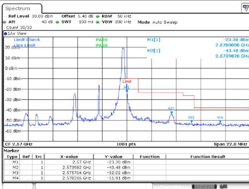
Band7-5MHz-QPSK-21425-1RB#24
