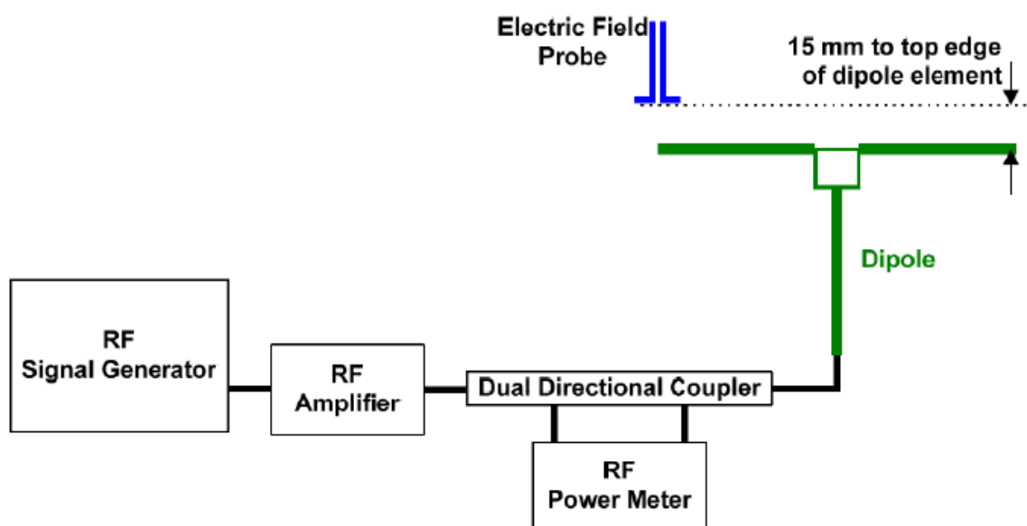
Fig.4 System verification
