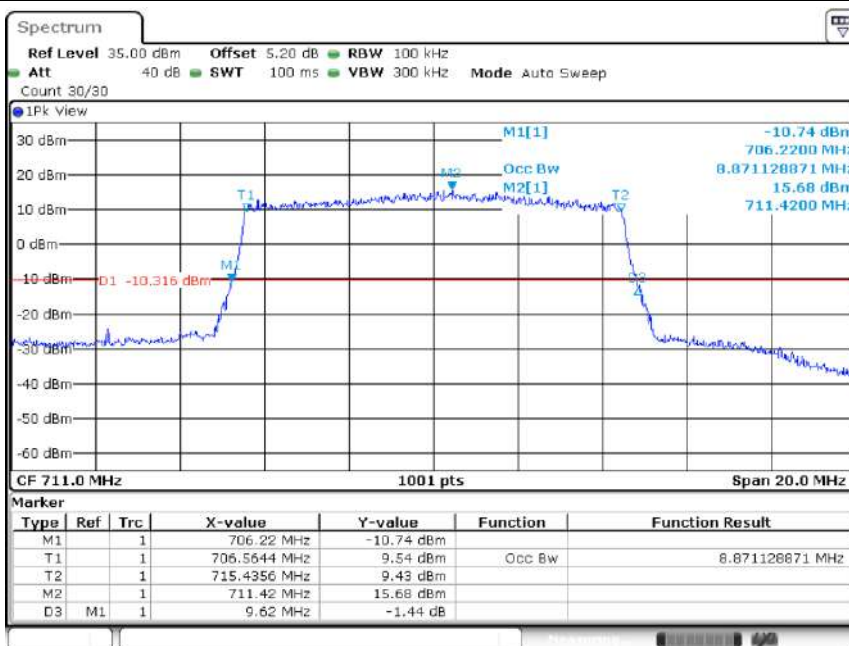
Band12-10MHz-16QAM-23130-50RB#0-8.871
