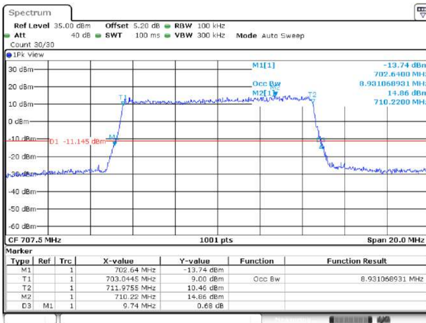
Band12-10MHz-16QAM-23095-50RB#0-8.931
