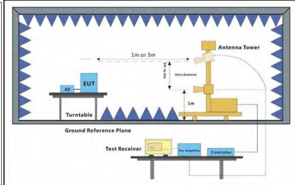
Figure 2. Above 1 GHz
