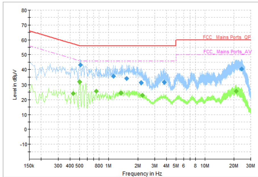
Fig.63 AC Power line Conducted Emission (Traffic), A2-2, A3-2
