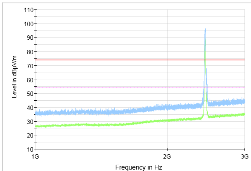
Fig.44 Radiated Spurious Emission (802.11g, CH6, 1 GHz-3 GHz)
