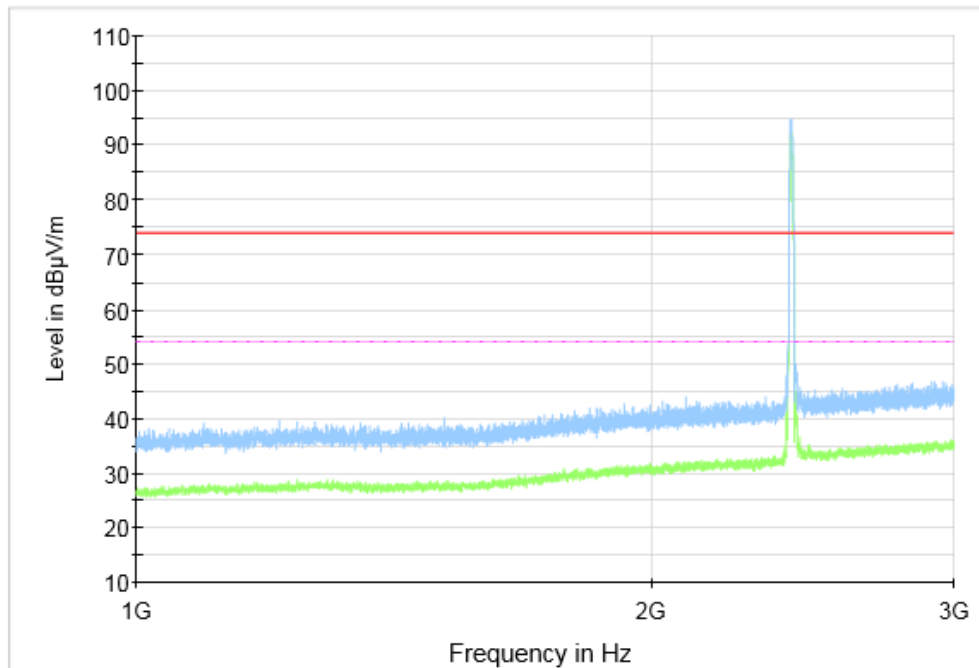
Fig.34 Radiated Spurious Emission (802.11b, CH1, 1 GHz-3 GHz)
