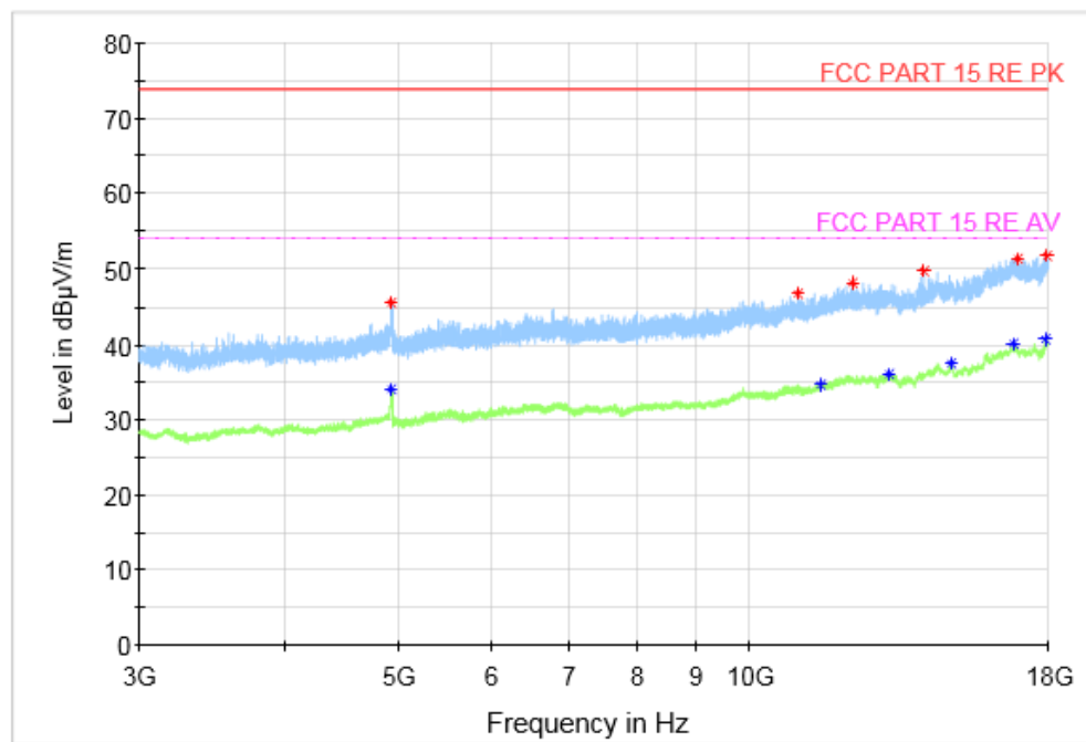
Fig.55 Radiated Spurious Emission (802.11n-HT20, CH11, 3 GHz-18 GHz)
