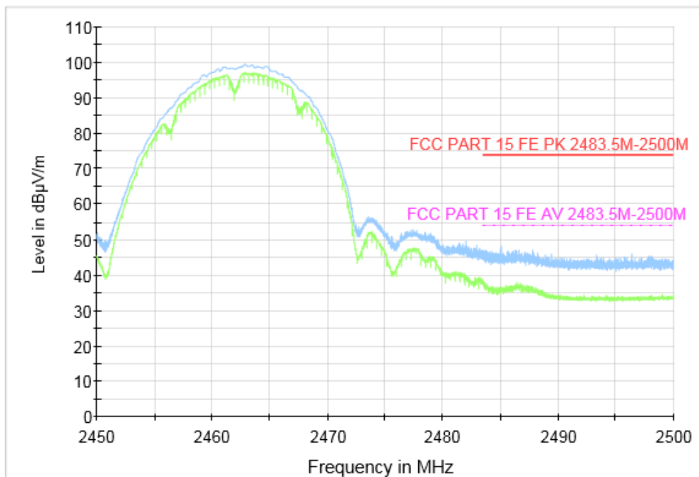
Fig.41 Radiated Restricted Band (802.11b, CH11, 2.45GHz~2.5GHz)
