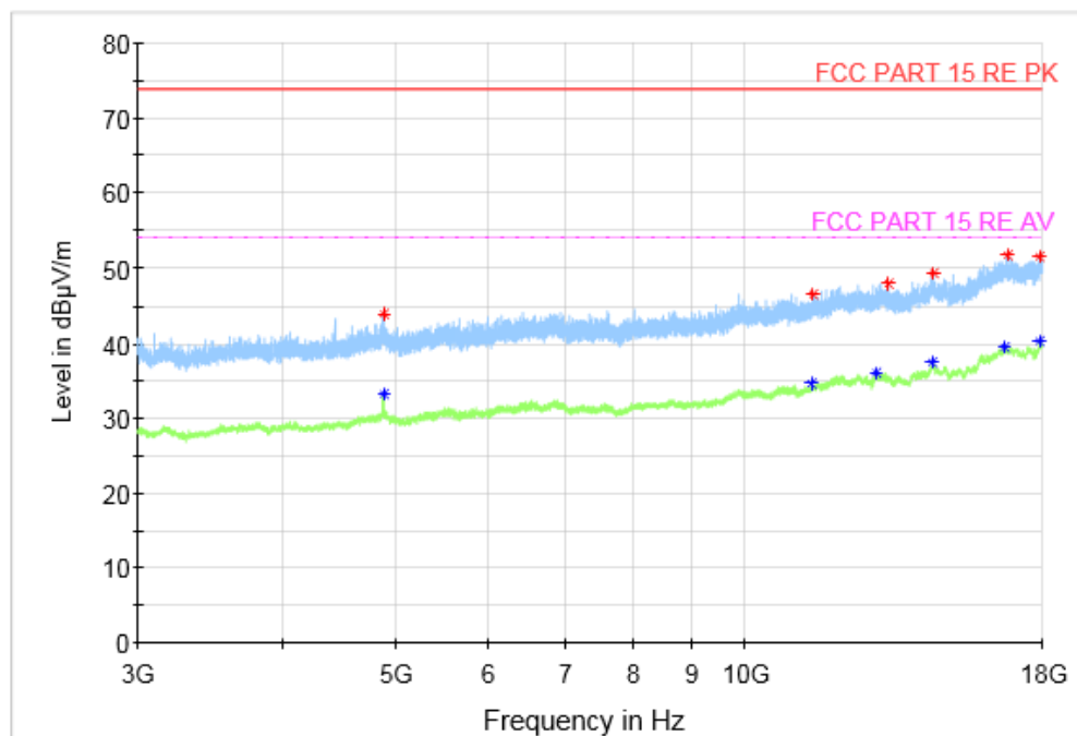
Fig.53 Radiated Spurious Emission (802.11n-HT20, CH6, 3 GHz-18 GHz)
