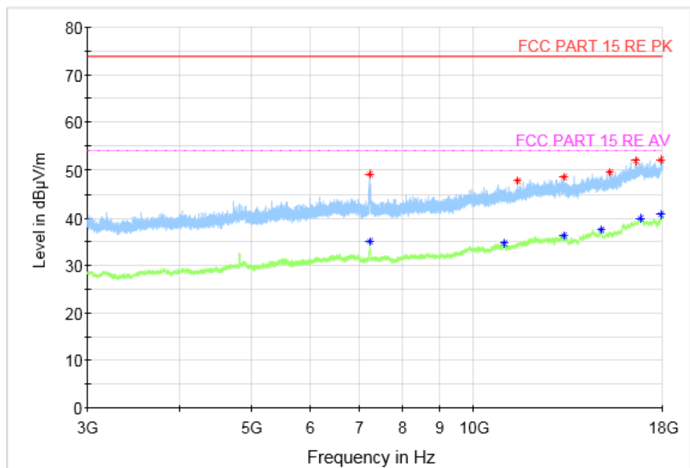
Fig.43 Radiated Spurious Emission (802.11g, CH1, 3 GHz-18 GHz)
