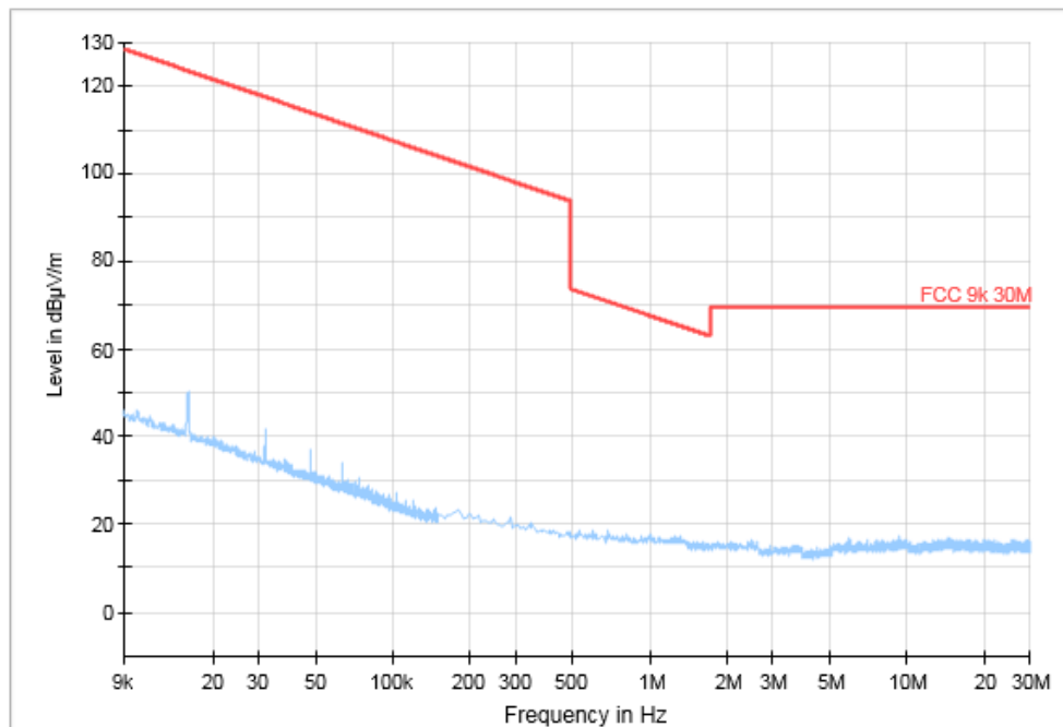
Fig.58 Radiated Spurious Emission (All Channels, 9 kHz-30 MHz)
