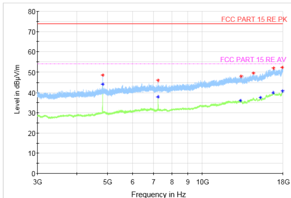
Fig.35 Radiated Spurious Emission (802.11b, CH1, 3 GHz-18 GHz)
