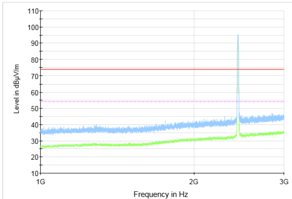
Fig.36 Radiated Spurious Emission (802.11b, CH6, 1 GHz-3 GHz)
