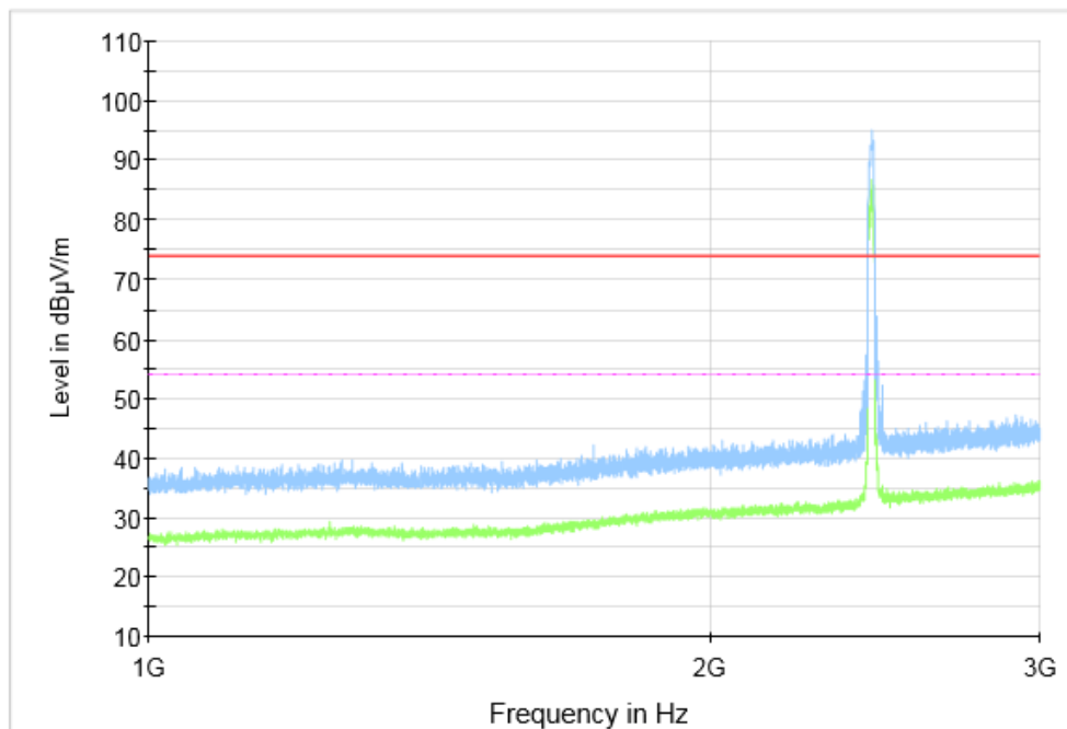
Fig.52 Radiated Spurious Emission (802.11n-HT20, CH6, 1 GHz-3 GHz)
