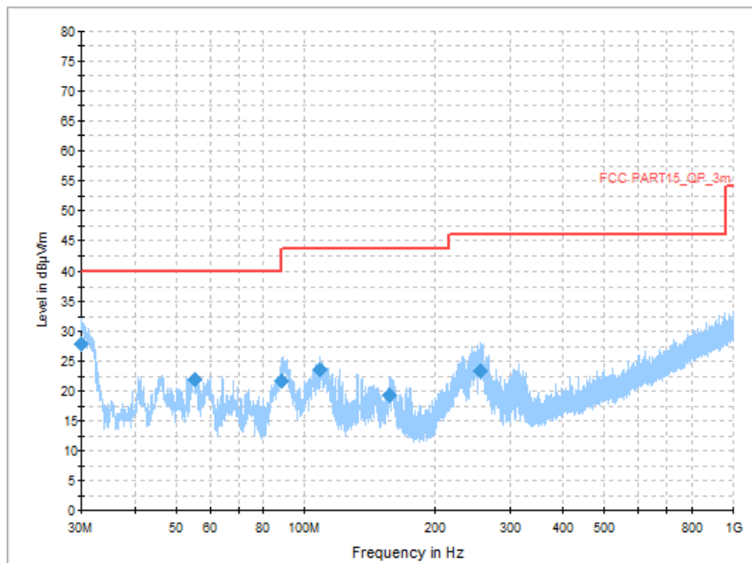
Fig.26 Radiated Spurious Emission (All Channels, 30 MHz-1 GHz)
