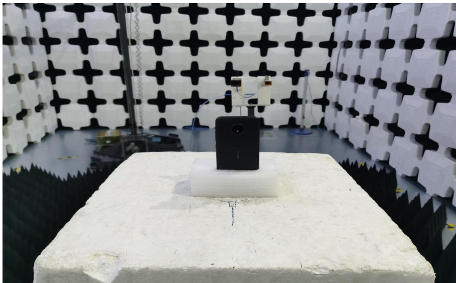
8. Radiated Emissions (Part 15C, 18GHz -26.5GHz)
