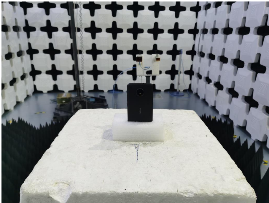
10. Radiated Emissions (Part 22/24/27, 18GHz -26.5GHz)
