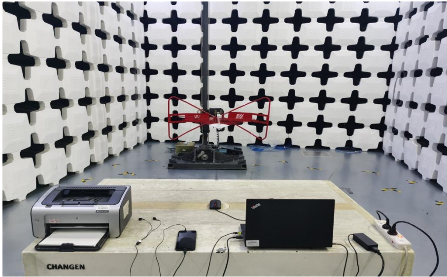
1. Radiated Emissions (Part 15B Data Transfer ,30MHz-1GHz)
