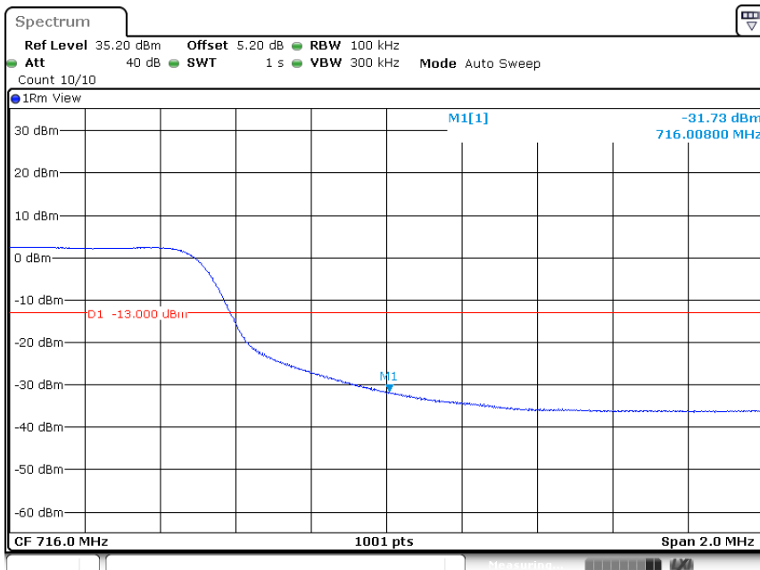
Band12-10MHz-QPSK-23130-50RB#0
