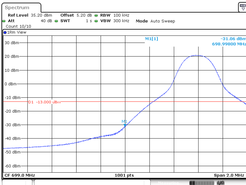
Band12-10MHz-16QAM-23060-1RB#0
