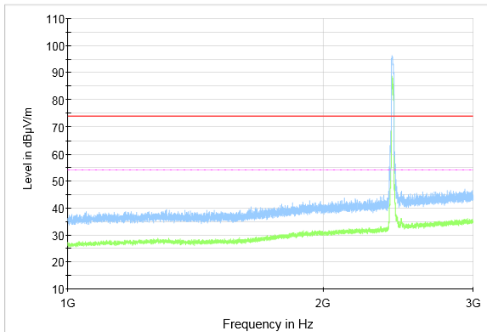
Fig.42 Radiated Spurious Emission (802.11g, CH1, 1 GHz-3 GHz)
