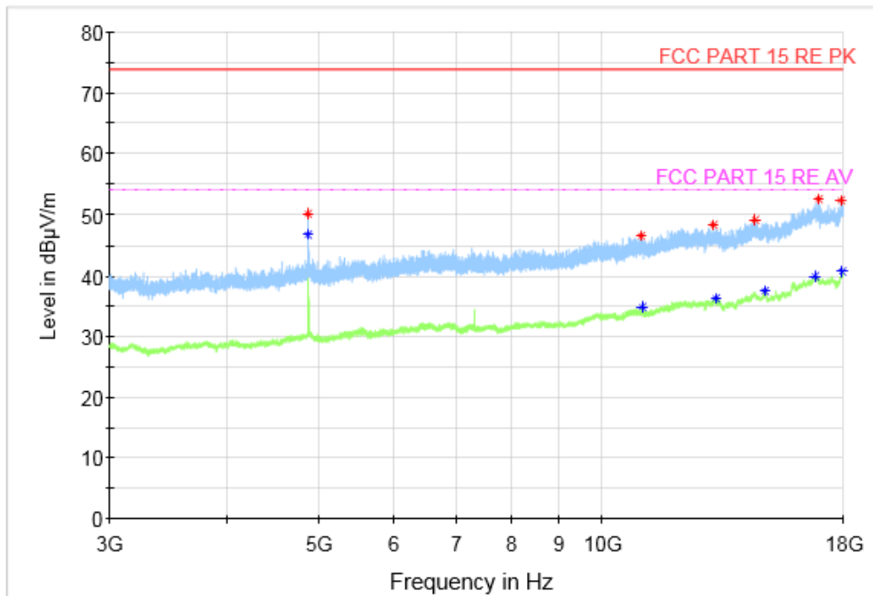
Fig.37 Radiated Spurious Emission (802.11b, CH6, 3 GHz-18 GHz)
