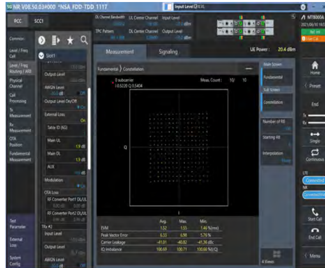
NTNV-DC_2A_n71A-15kHz-5MHz+20MHz-N/A+DFT-256QAM-Mid+Mid-N/A-Outer_Full-----±2.5ppm-PASS
