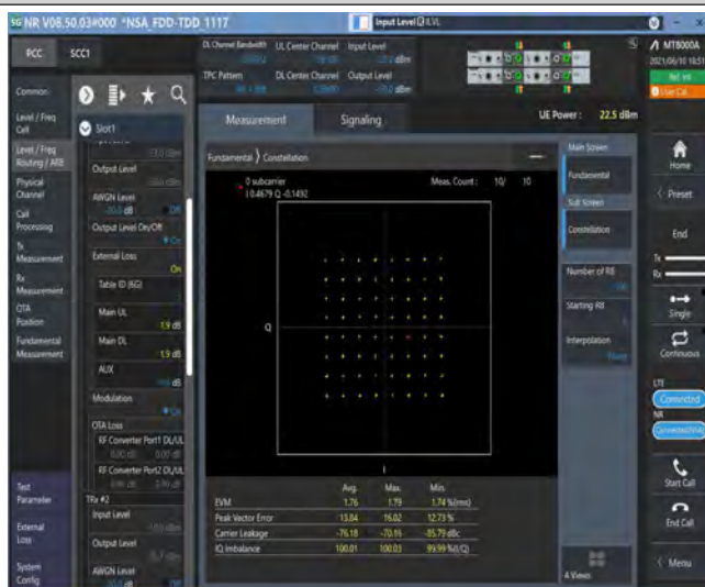
NTNV-DC_2A_n71A-15kHz-5MHz+20MHz-N/A+DFT-64QAM-Mid+Mid-N/A-Outer_Full-----±2.5ppm-PASS
