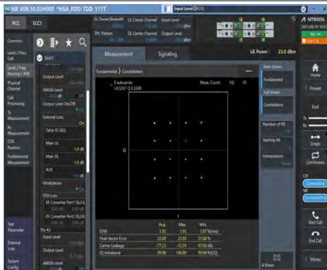
NTNV-DC_2A_n71A-15kHz-5MHz+20MHz-N/A+DFT-16QAM-Mid+Mid-N/A-Outer_Full-----±2.5ppm-PASS
