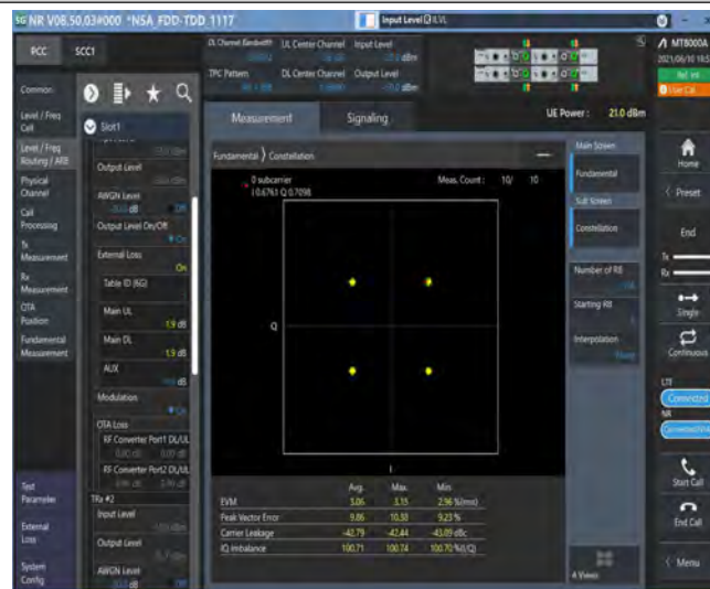
NTNV-DC_2A_n71A-15kHz-5MHz+20MHz-N/A+CP-QPSK-Mid+Mid-N/A-Outer_Full-----±2.5ppm-PASS
