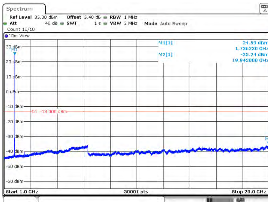
Band4-20MHz-16QAM-20300-1RB#0-Range2:1000~20000MHz
