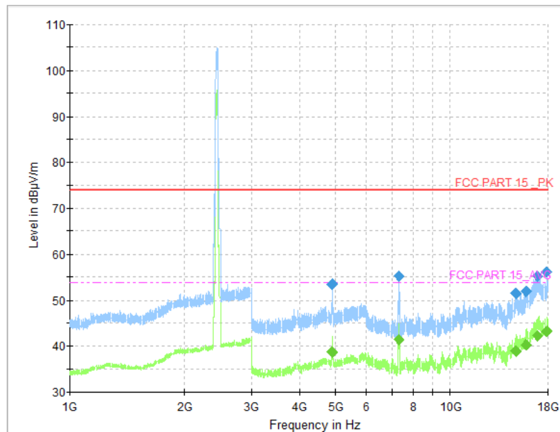
Fig.85 Radiated Spurious Emission (802.11n-HT40, CH6, 1 GHz-18 GHz)
