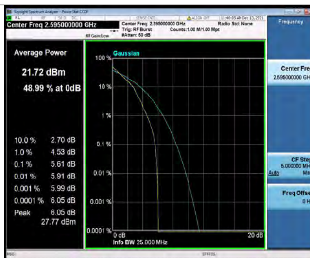
Band38-10MHz-64QAM-38000-50RB#0
