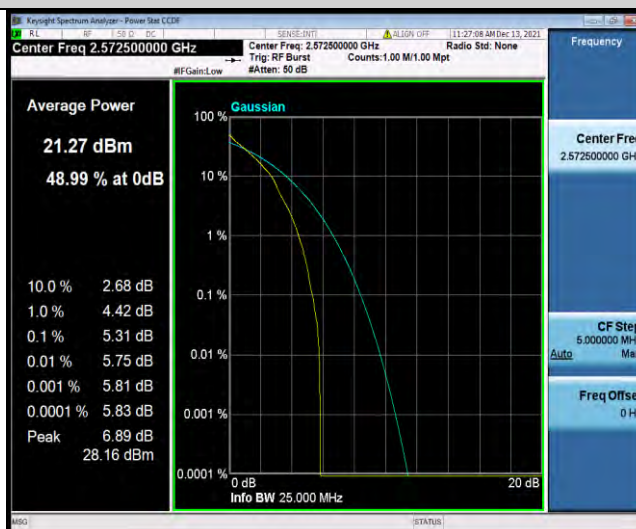
Band38-5MHz-64QAM-37775-25RB#0
