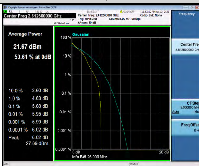
Band38-15MHz-64QAM-38175-75RB#0
