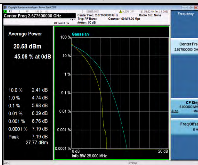
Band38-15MHz-64QAM-38000-1RB#0
