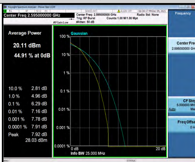
Band38-20MHz-16QAM-38150-1RB#0
