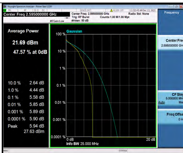
Band38-15MHz-64QAM-38000-75RB#0
