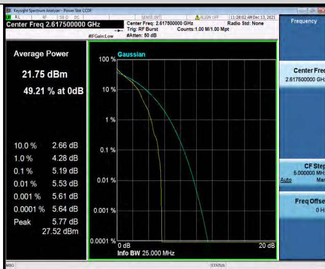
Band38-5MHz-64QAM-38225-25RB#0
