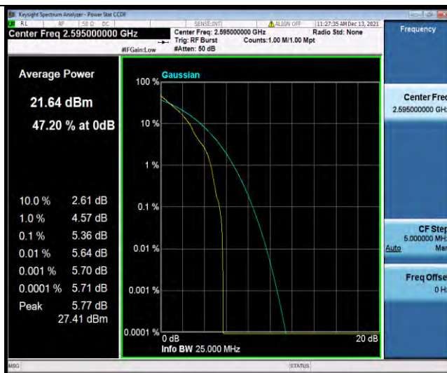
Band38-5MHz-64QAM-38000-25RB#0
