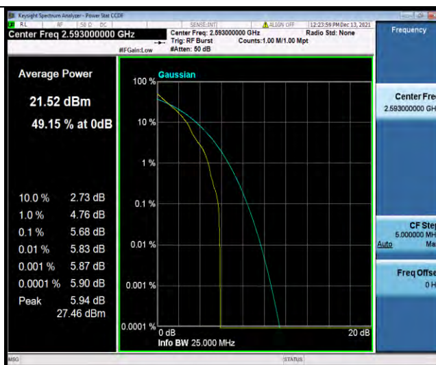
Band41-5MHz-64QAM-40620-25RB#0
