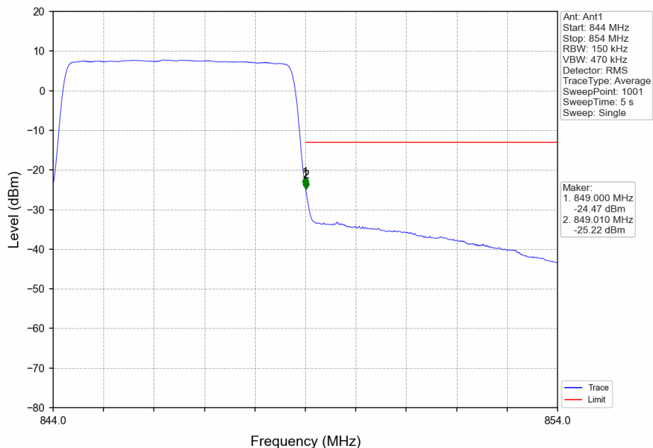
Band5_5MHz_16QAM_HCH_846.5MHz_RB_25_0_NTNV
