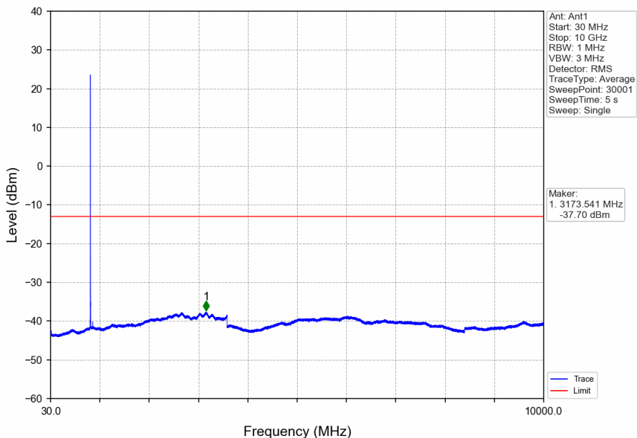
Band5_3MHz_QPSK_MCH_836.5MHz_RB_1_0_NTNV
