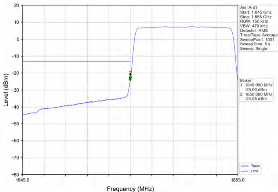
Band2_5MHz_16QAM_LCH_1852.5MHz_RB_25_0_NTNV
