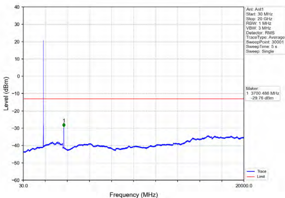
Band2_5MHz_16QAM_LCH_1852.5MHz_RB_25_0_NTNV
