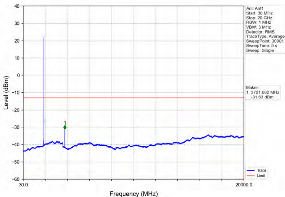
Band2_15MHz_64QAM_HCH_1902.5MHz_RB_1_74_NTNV
