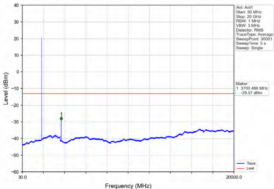
Band2_3MHz_64QAM_LCH_1851.5MHz_RB_1_0_NTNV
