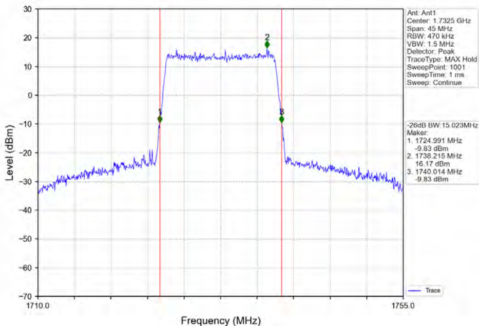
Band4 15MHz 64QAM MCH 1732.5MHz RB 75_0 NTVN
