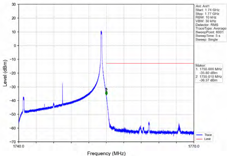
Band4_15MHz_64QAM_HCH_1747.5MHz_RB_1_74_NTNV
