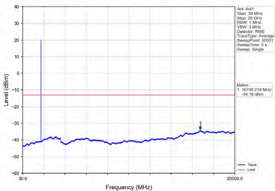
Band4_5MHz_64QAM_HCH_1752.5MHz_RB_1_24_NTNV
