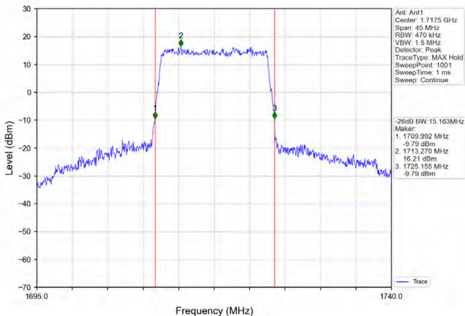
Band4 15MHz 16QAM LCH 1717.5MHz RB 75 0 NTNV
