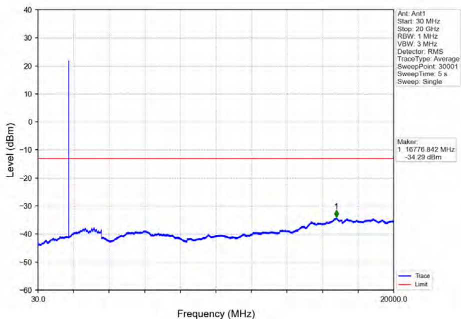
Band4 1.4MHz QPSK HCH 1754.3MHz RB 1 5 NTNV
