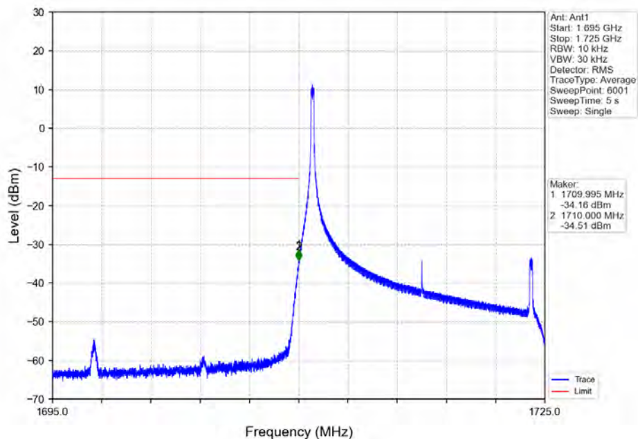
Band4 15MHz 16QAM LCH 1717.5MHz RB 1 0 NTNV
