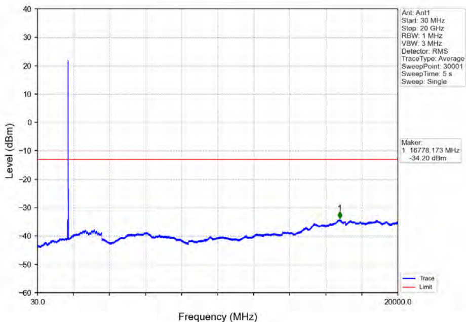
Band4_15MHz_QPSK_MCH_1732.5MHz_RB_1_0_NTNV
