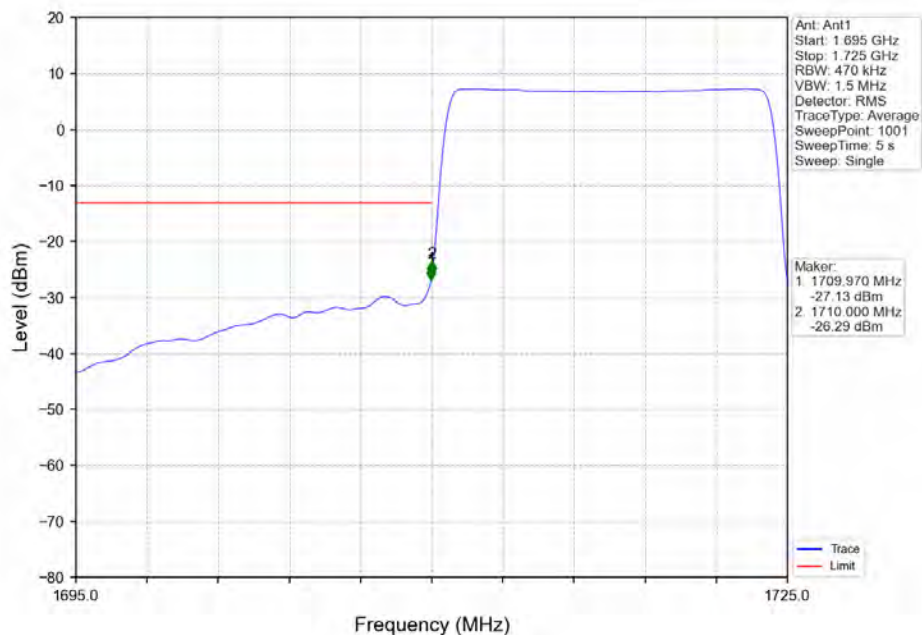
Band4_15MHz_16QAM_LCH_1717.5MHz_RB_75_0_NTNV
