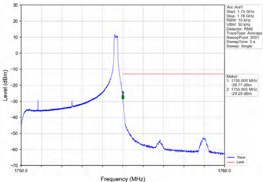
Band4_5MHz_QPSK_HCH_1752.5MHz_RB_1_24_NTNV
