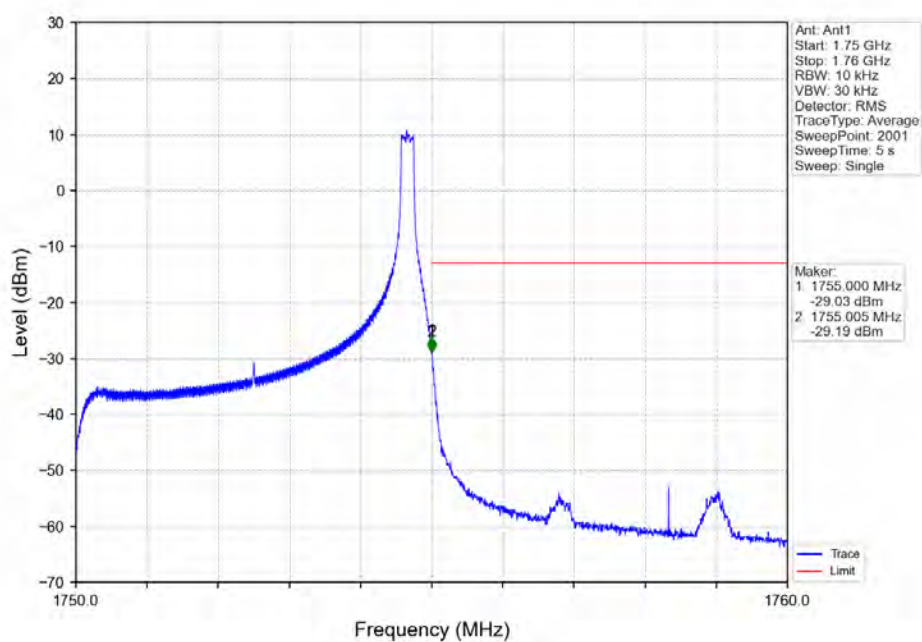
Band4_5MHz_16QAM_HCH_1752.5MHz_RB_25_0_NTNV
