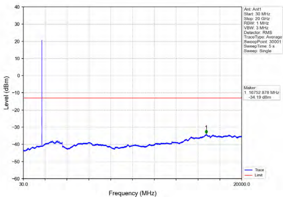
Band4_3MHz_16QAM_HCH_1753.5MHz_RB_1_0_NTNV
