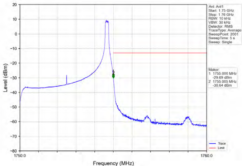
Band4_5MHz_64QAM_HCH_1752.5MHz_RB_1_24_NTNV
