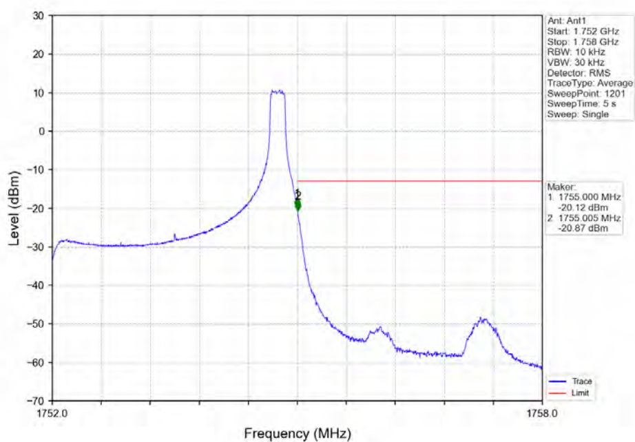
Band4_3MHz_16QAM_HCH_1753.5MHz_RB_15_0_NTNV
