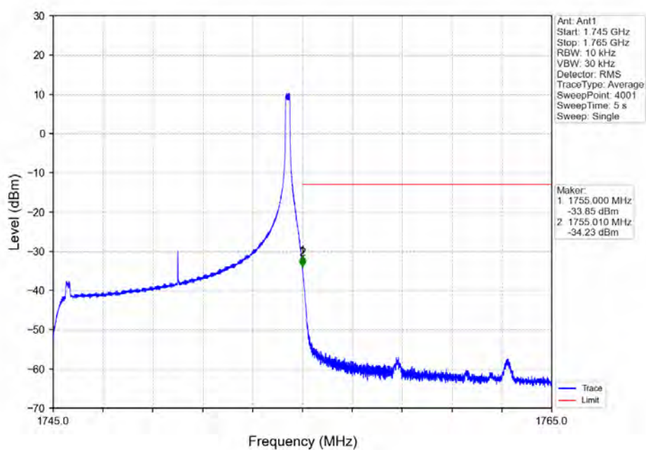
Band4_10MHz_16QAM_HCH_1750MHz_RB_50_0_NTNV
