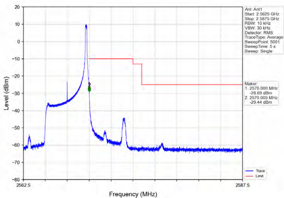
Band7_5MHz_16QAM_HCH_2567.5MHz_RB_25_0_NTNV
