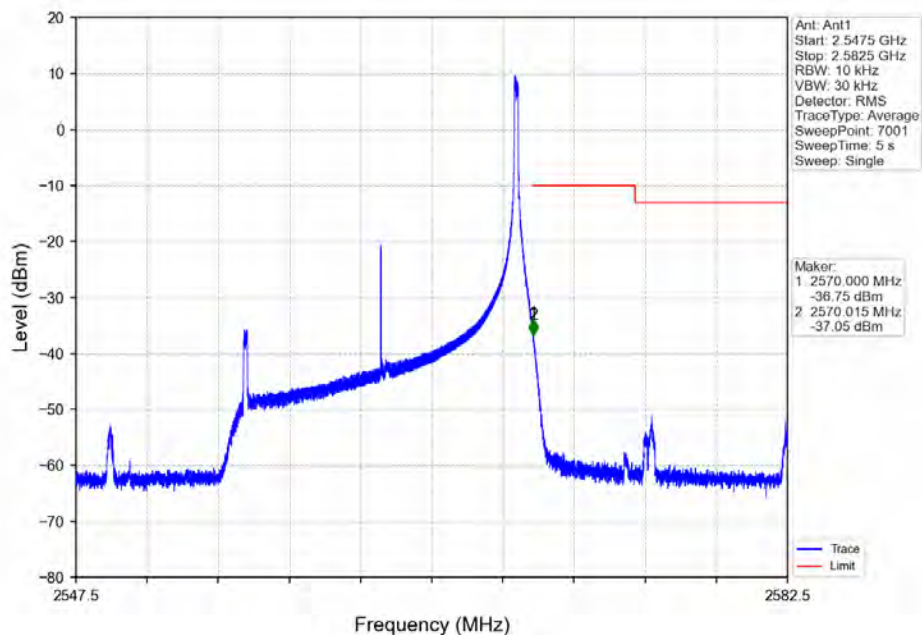
Band7_15MHz_64QAM_HCH_2562.5MHz_RB_1_74_NTNV
