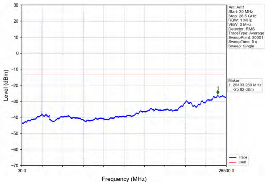
Band7 5MHz 64QAM MCH 2535MHz RB 1 0 NTV
