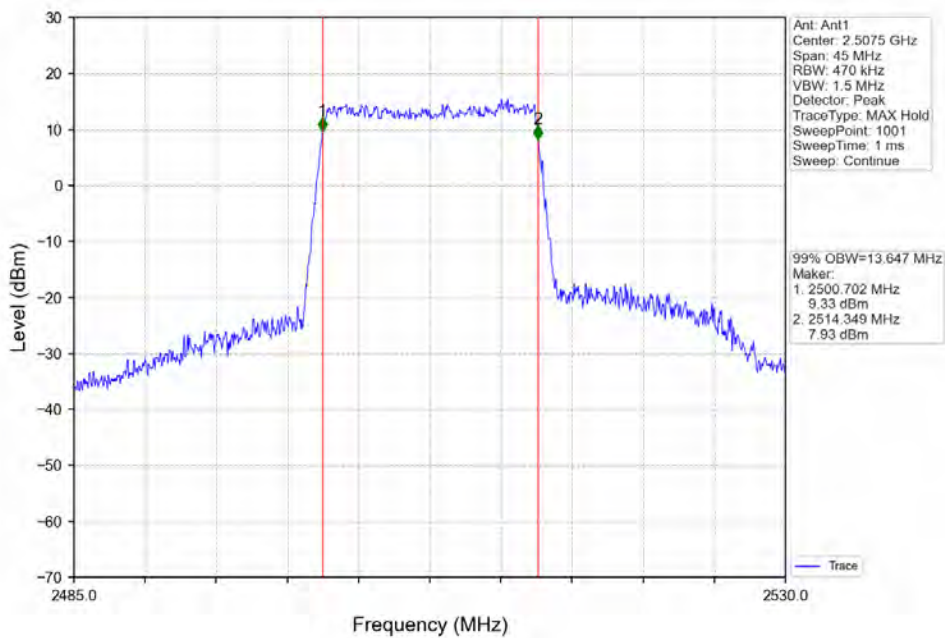
Band7 15MHz 16QAM LCH 2507.5MHz RB 75 0 NTN
