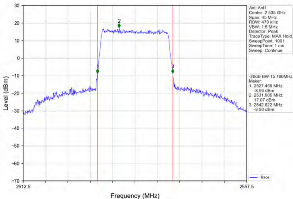
Band7 15MHz QPSK MCH 2535MHz RB 75 0 NTNV
