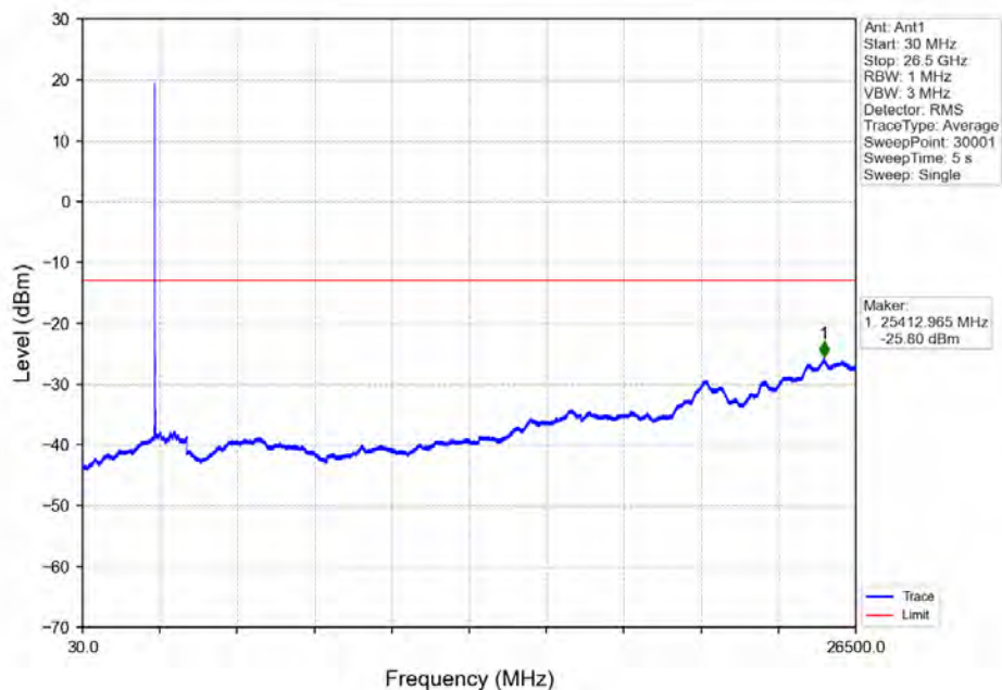
Band7 15MHz 64QAM LCH 2507.5MHz RB 1 0 NTVN
