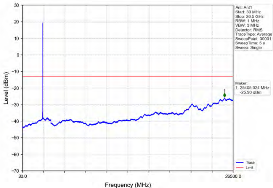
Band7_10MHz_64QAM_MCH_2535MHz_RB_1_0_NTNV
