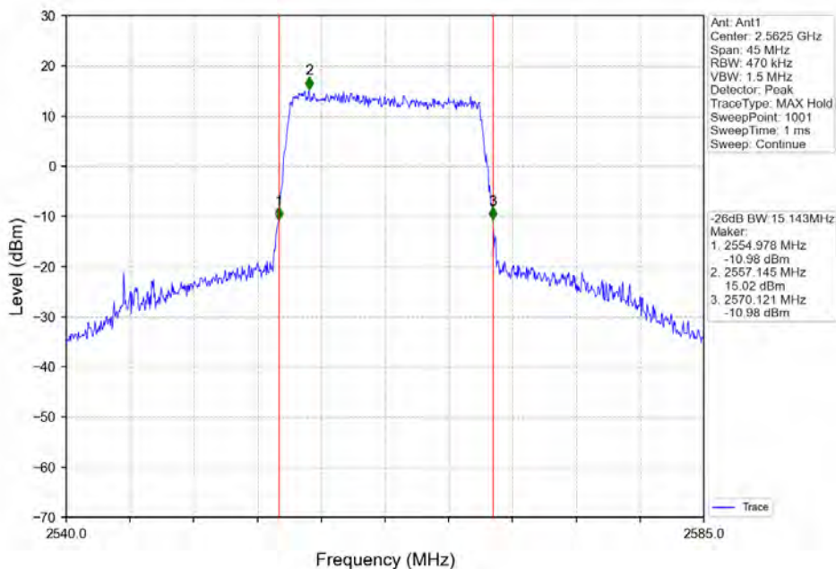
Band7 15MHz 16QAM HCH 2562.5MHz RB 75 0 NTVN
