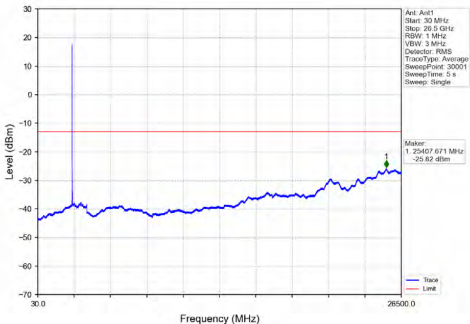
Band7 15MHz 64QAM MCH 2535MHz RB 1 0 NTNV
