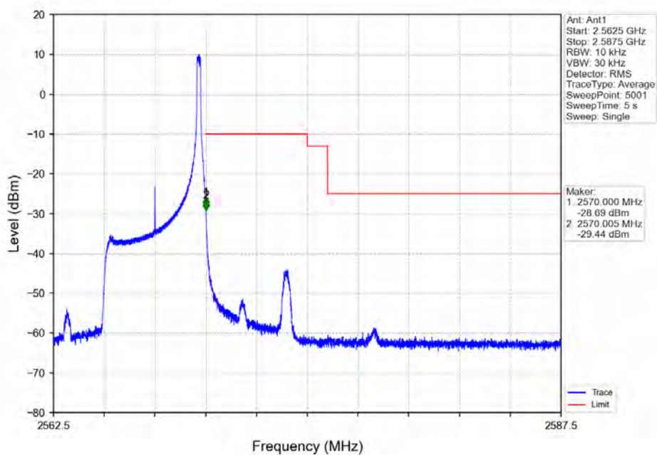
Band7_5MHz_16QAM_HCH_2567.5MHz_RB_25_0_NTNV
