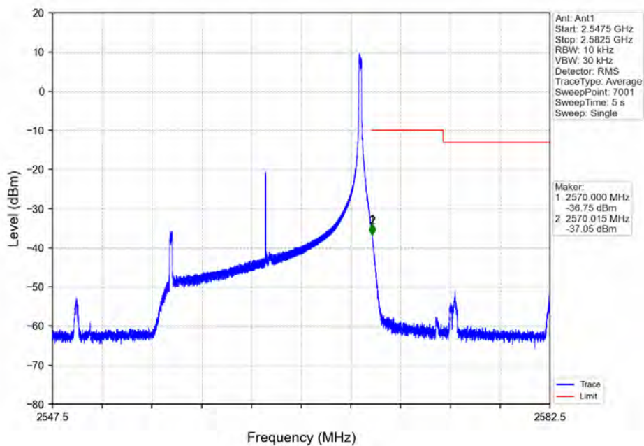
Band7_15MHz_64QAM_HCH_2562.5MHz_RB_1_74_NTNV
