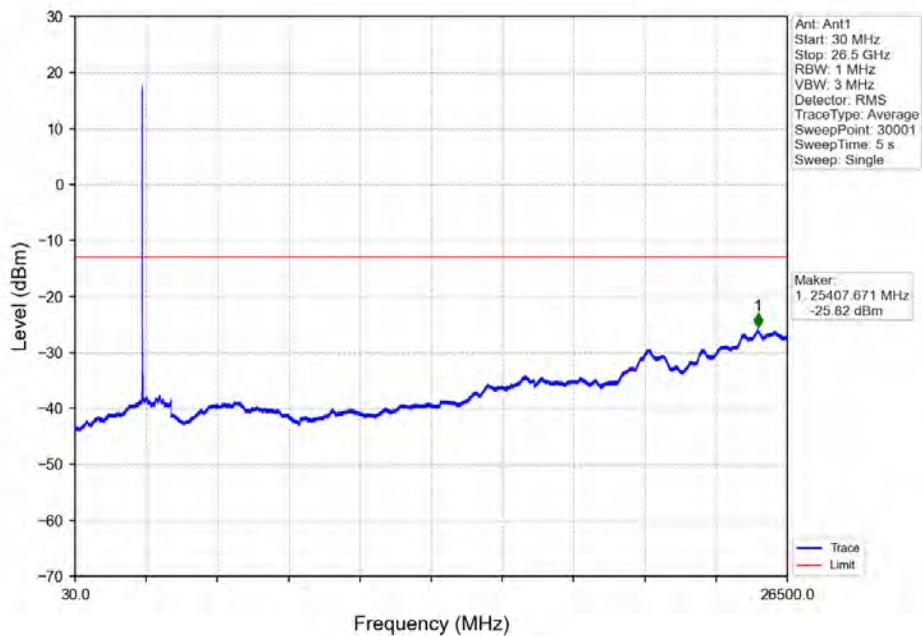
Band7_15MHz_64QAM_MCH_2535MHz_RB_1_0_NTNV
