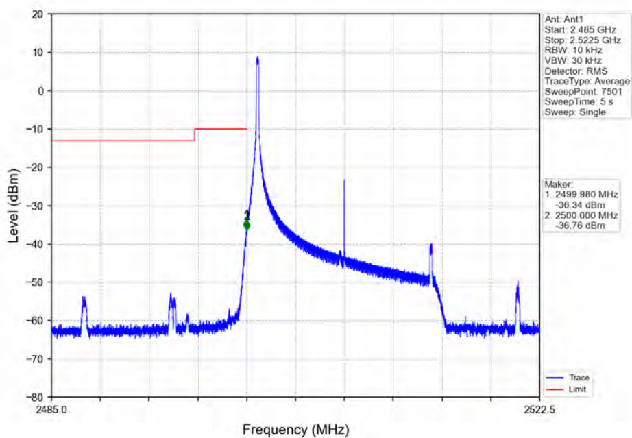
Band7 15MHz 64QAM LCH 2507.5MHz RB 1 0 NTNV
