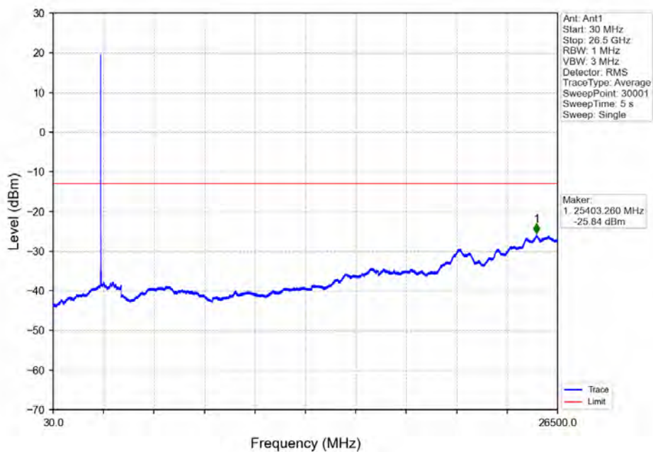
Band7 15MHz QPSK MCH 2535MHz RB 1 0 NTNV
