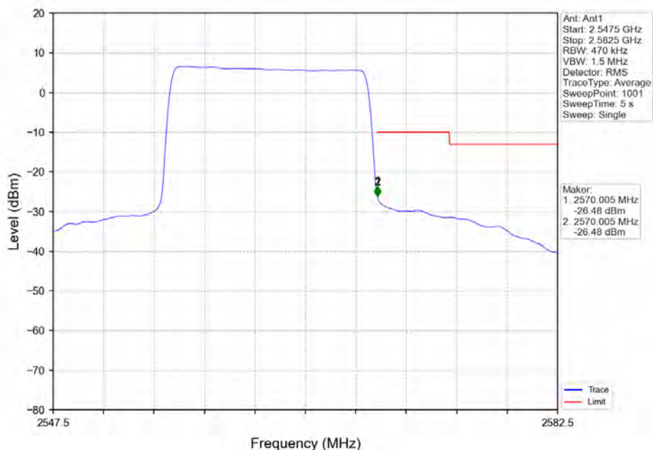
Band7 15MHz 16QAM HCH 2562.5MHz RB 75 0 NTV
