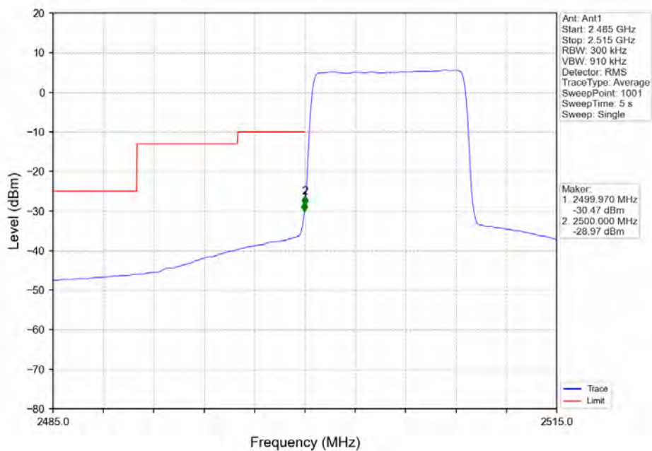
Band7_10MHz_16QAM_LCH_2505MHz_RB_50_0_NTNV
