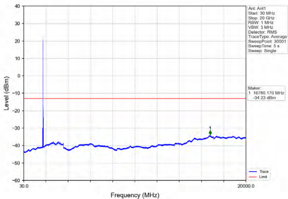
Band66_20MHz_64QAM_HCH_1770MHz_RB_1_99_NTNV
