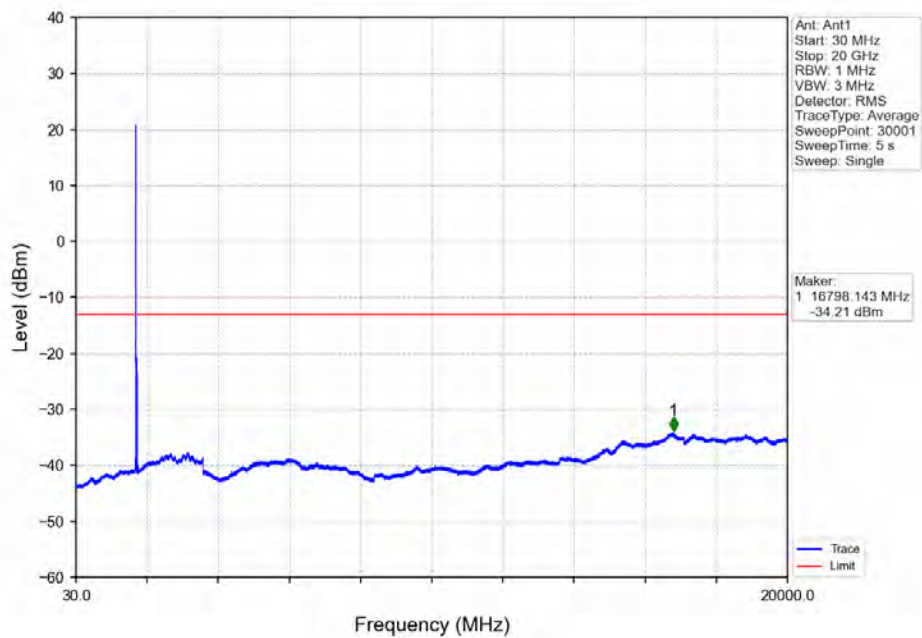
Band66_20MHz_64QAM_LCH_1720MHz_RB_1_0_NTNV
