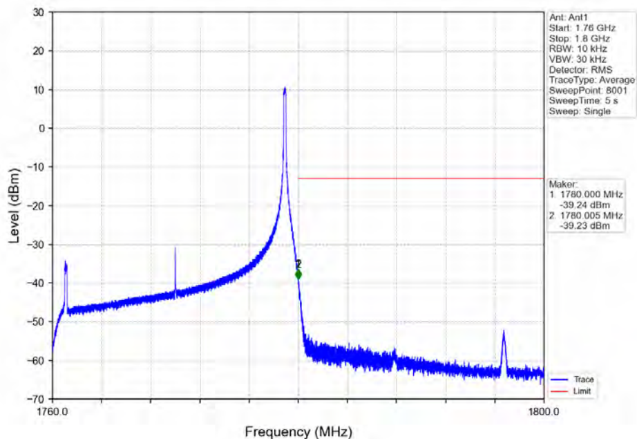
Band66_20MHz_64QAM_HCH_1770MHz_RB_1_99_NTNV
