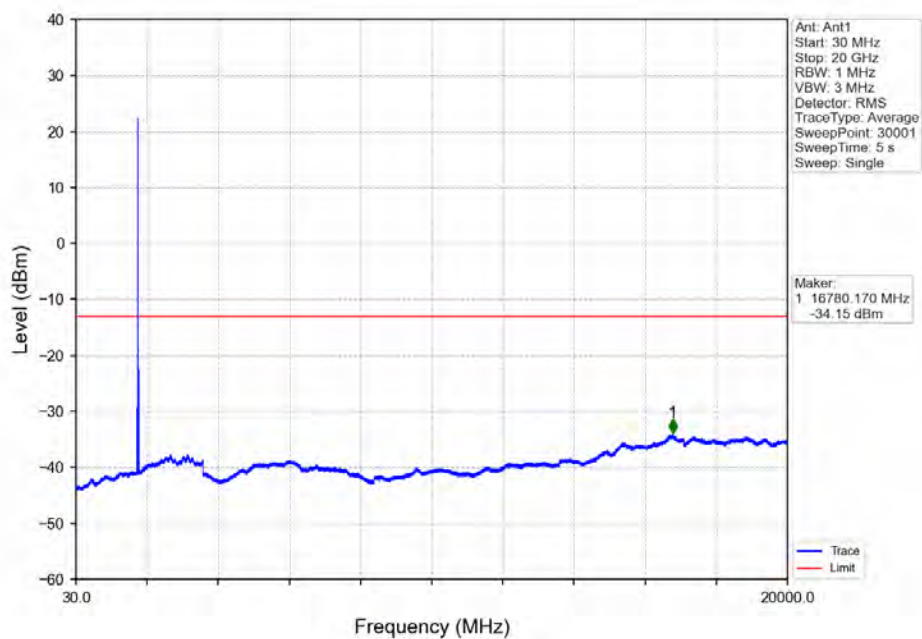
Band66_15MHz_QPSK_HCH_1772.5MHz_RB_1_74_NTNV
