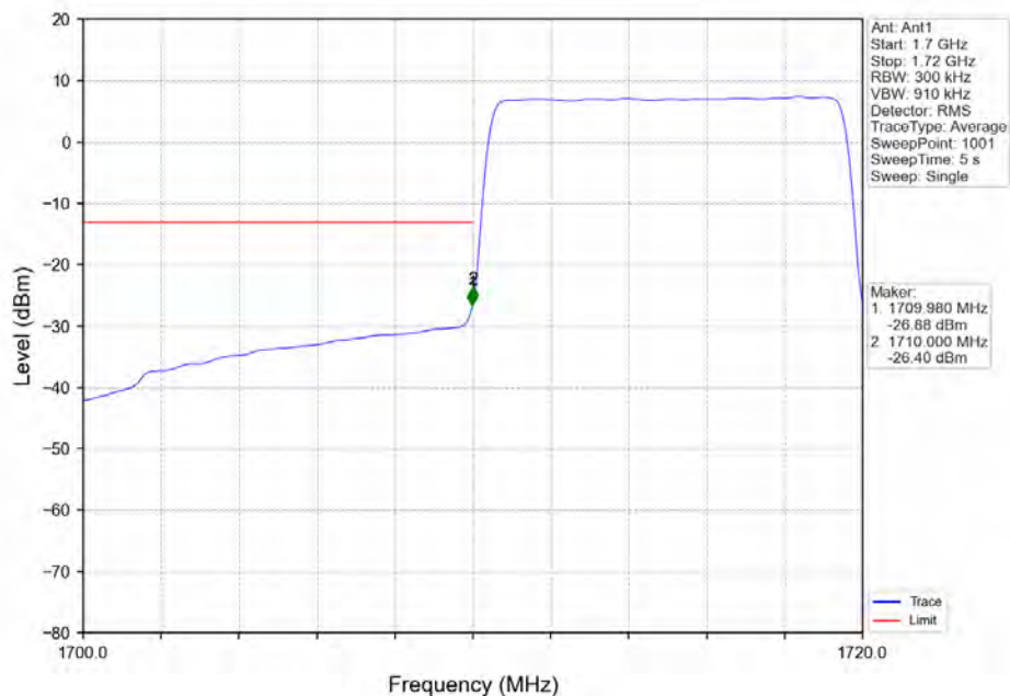
Band66_10MHz_16QAM_LCH_1715MHz_RB_50_0_NTNV
