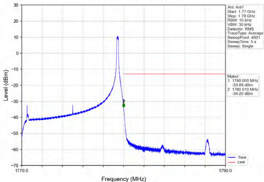
Band66_10MHz_64QAM_HCH_1775MHz_RB_1_49_NTNV
