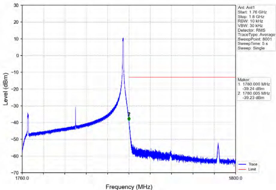
Band66_20MHz_64QAM_HCH_1770MHz_RB_1_99_NTNV
