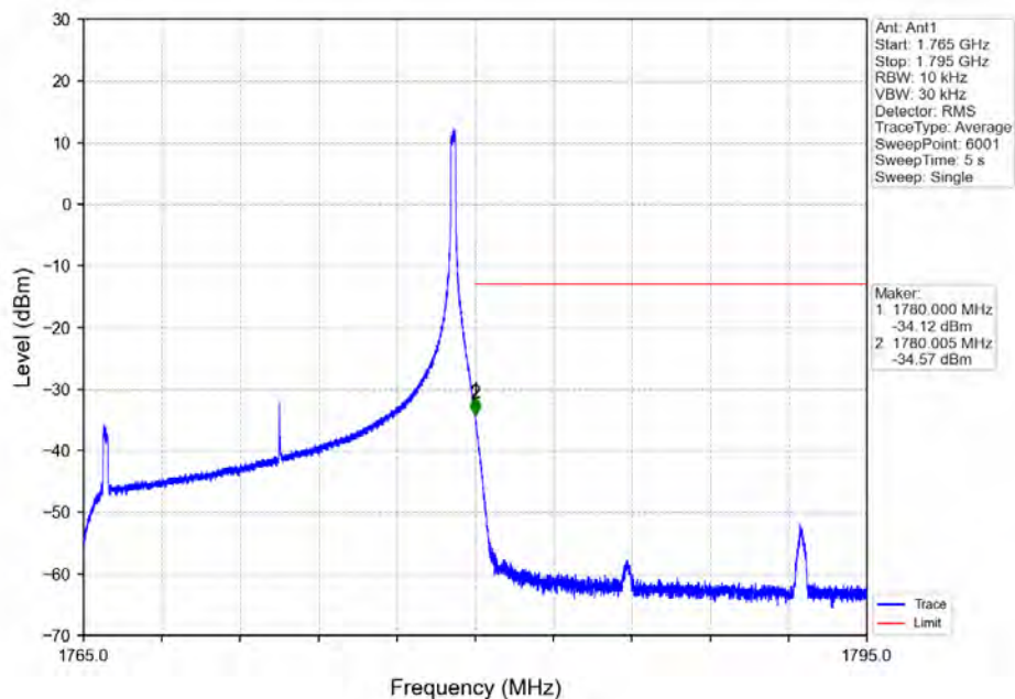
Band66_15MHz_QPSK_HCH_1772.5MHz_RB_1_74_NTNV
