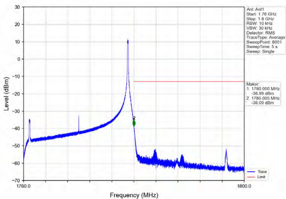
Band66_20MHz_16QAM_HCH_1770MHz_RB_100_0_NTNV
