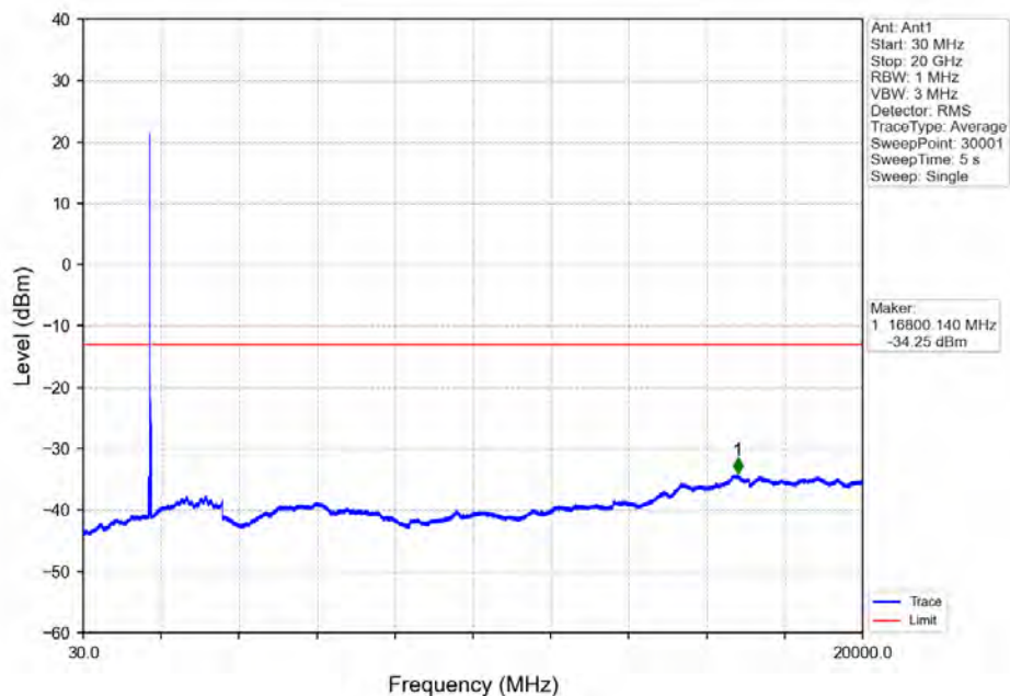
Band66_20MHz_64QAM_MCH_1745MHz_RB_1_0_NTNV
