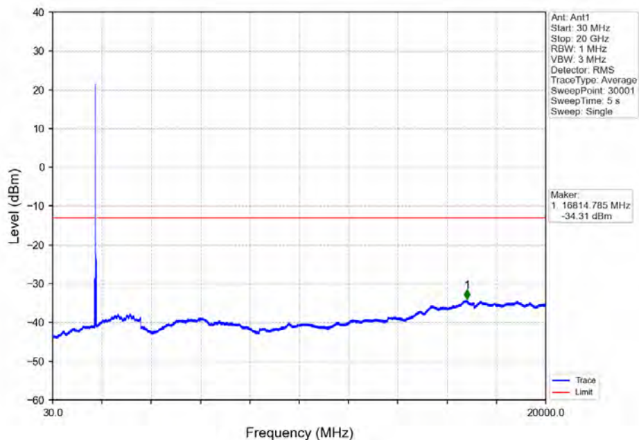
Band66_20MHz_16QAM_HCH_1770MHz_RB_1_0_NTNV
