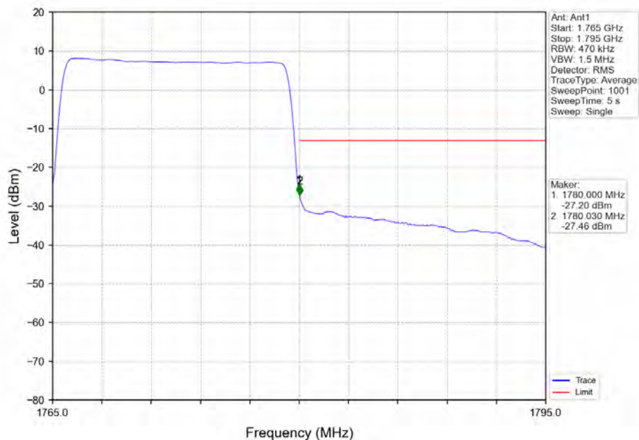
Band66_15MHz_16QAM_HCH_1772.5MHz_RB_75_0_NTNV
