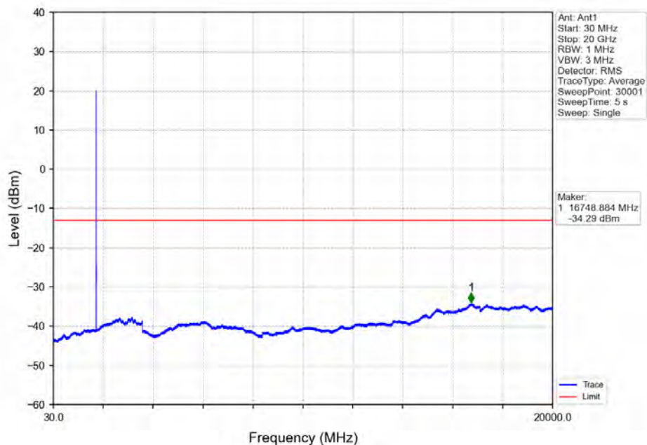
Band66_3MHz_64QAM_MCH_1745MHz_RB_1_0_NTNV
