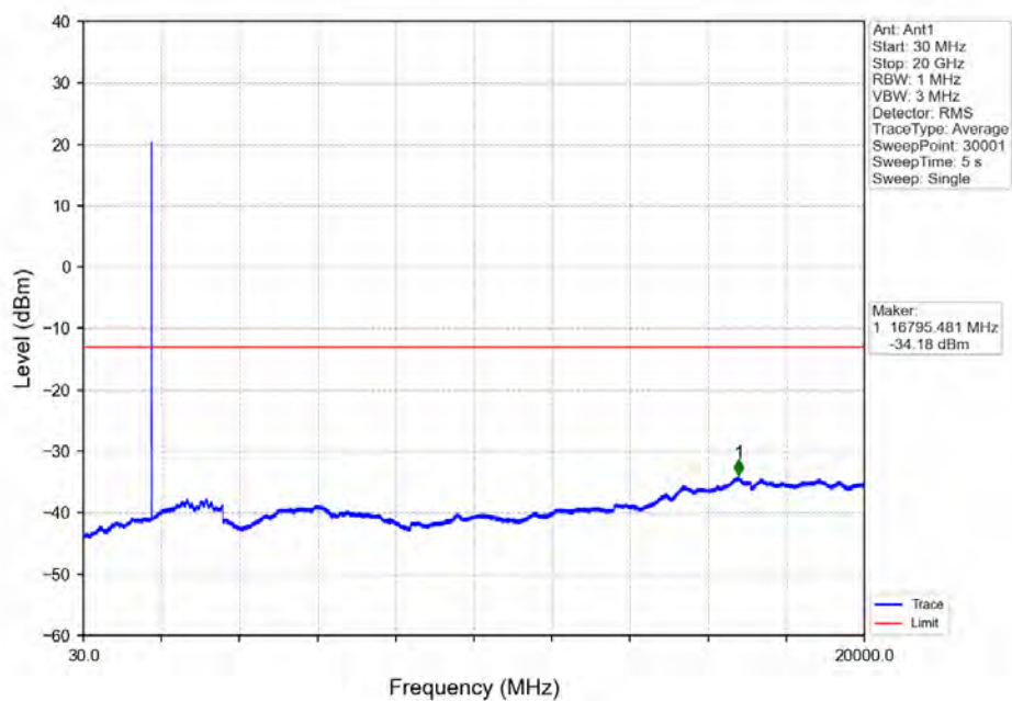
Band66_3MHz_64QAM_HCH_1778.5MHz_RB_1_14_NTNV
