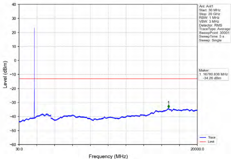
Band66_5MHz_QPSK_MCH_1745MHz_RB_1_0_NTNV
