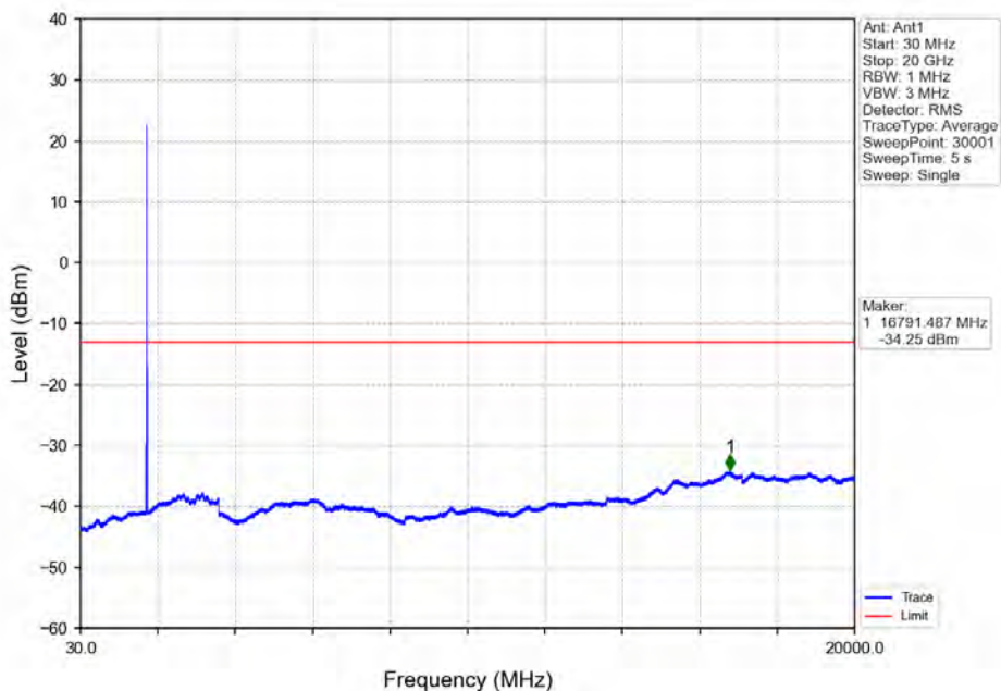
Band66_10MHz_QPSK_MCH_1745MHz_RB_1_0_NTNV
