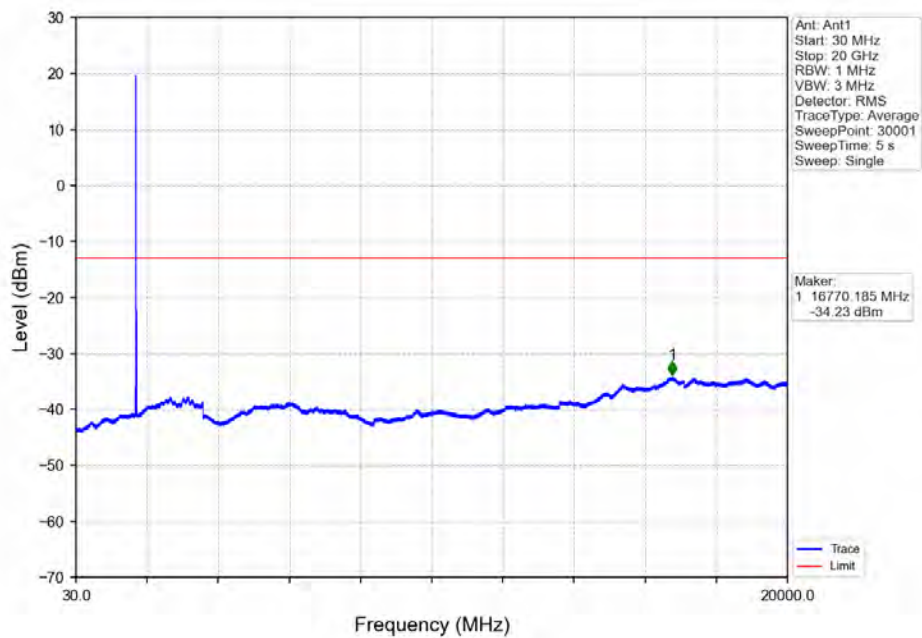
Band66_10MHz_64QAM_LCH_1715MHz_RB_1_0_NTNV
