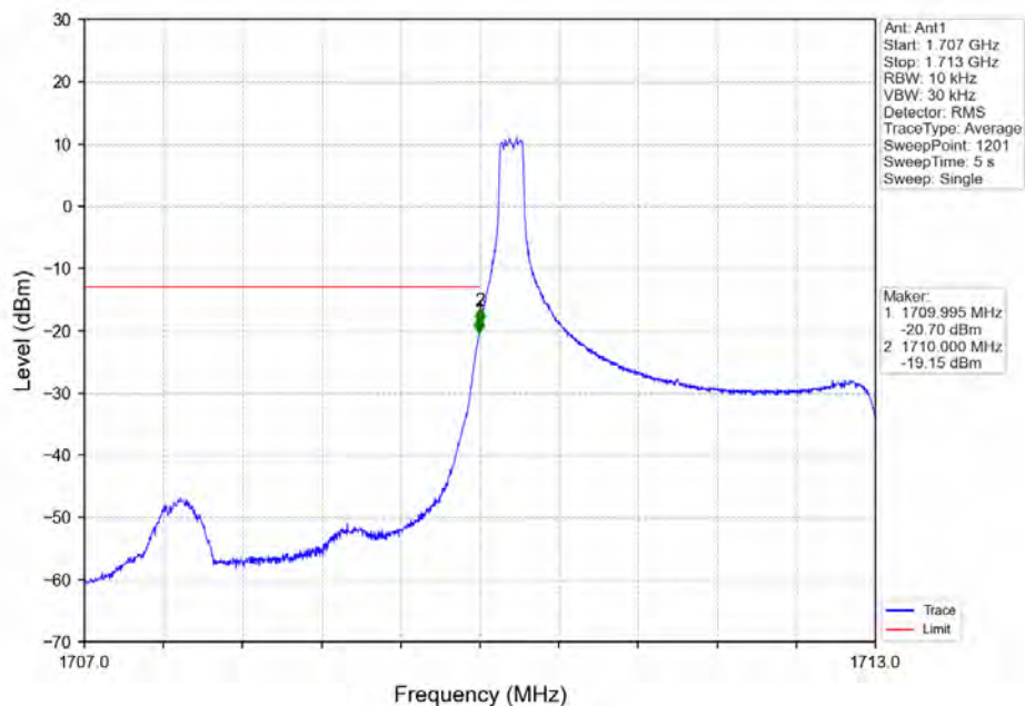
Band66_3MHz_16QAM_LCH_1711.5MHz_RB_1_0_NTNV
