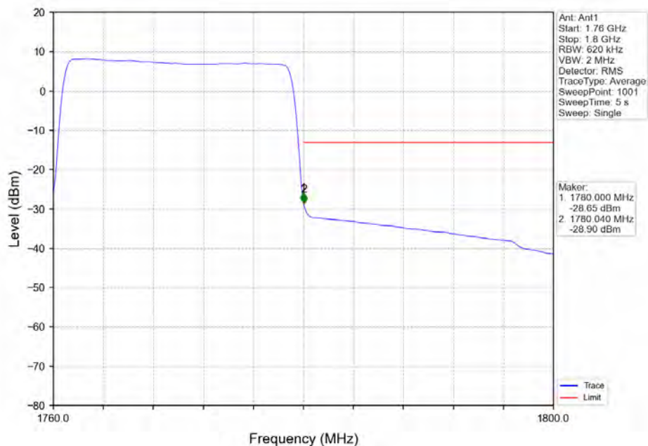
Band66_20MHz_16QAM_HCH_1770MHz_RB_100_0_NTNV
