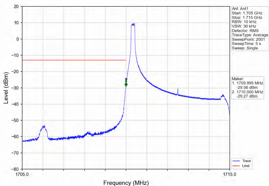
Band66_5MHz_64QAM_LCH_1712.5MHz_RB_1_0_NTNV
