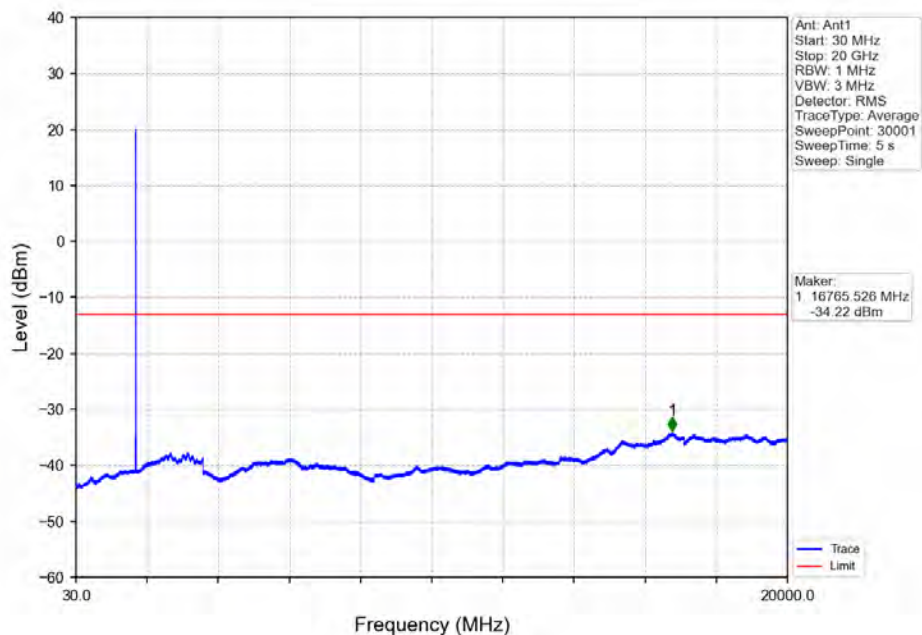
Band66_5MHz_64QAM_LCH_1712.5MHz_RB_1_0_NTNV
