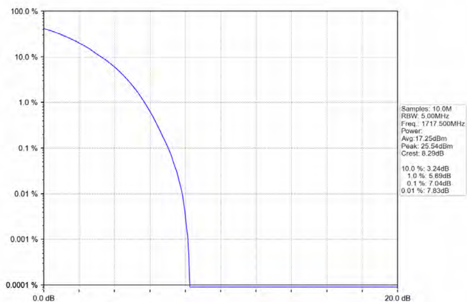
Band66_15MHz_64QAM_LCH_1717.5MHz_RB_75_0_NTNV
