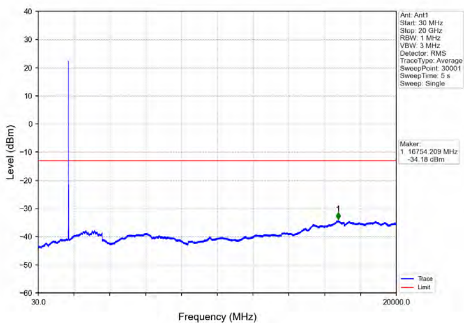
Band66_15MHz_16QAM_LCH_1717.5MHz_RB_75_0_NTNV
