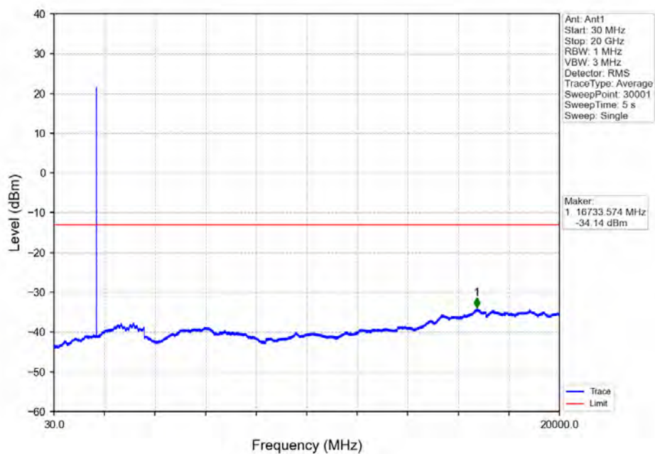
Band66_1.4MHz_16QAM_LCH_1710.7MHz_RB_6_0_NTNV
