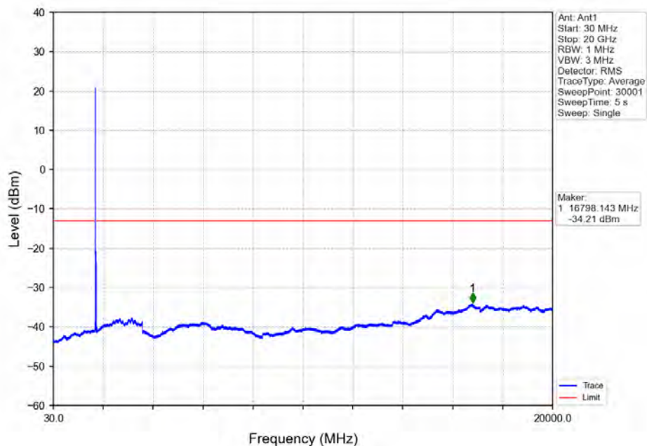
Band66_20MHz_64QAM_LCH_1720MHz_RB_1_0_NTNV
