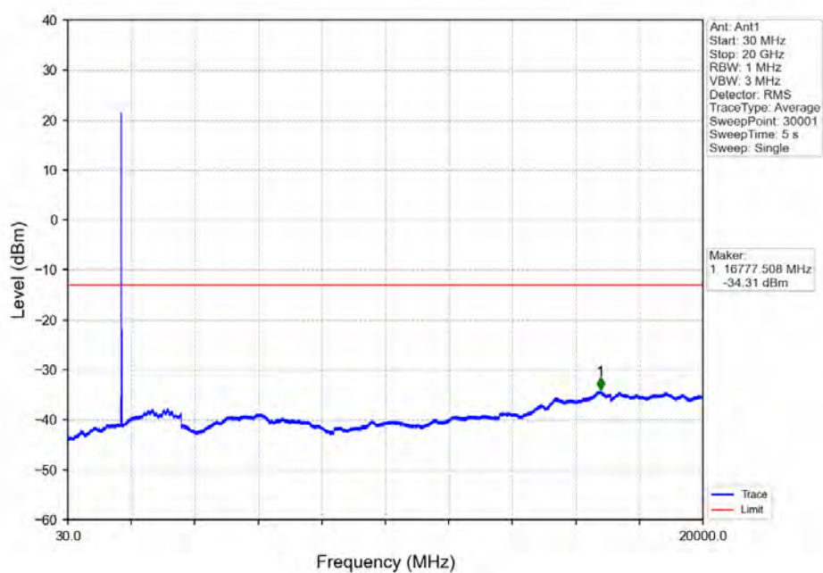
Band66_10MHz_16QAM_LCH_1715MHz_RB_50_0_NTNV
