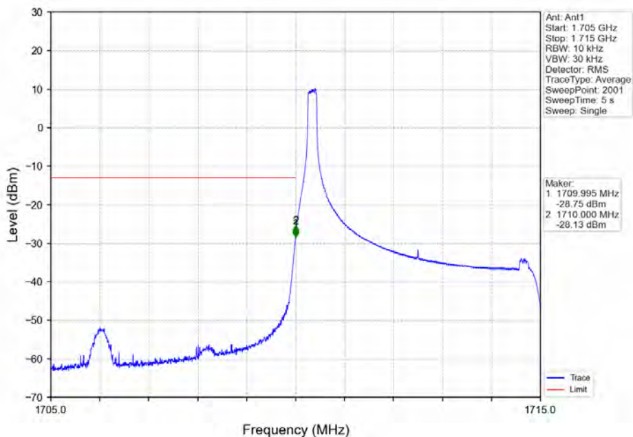
Band66_5MHz_16QAM_LCH_1712.5MHz_RB_1_0_NTNV
