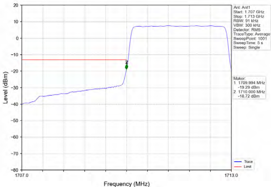
Band66_3MHz_16QAM_LCH_1711.5MHz_RB_15_0_NTNV
