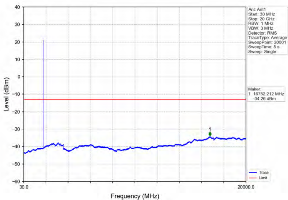
Band66_1.4MHz_64QAM_HCH_1779.3MHz_RB_1_5_NTNV
