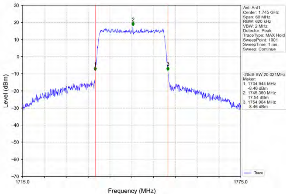
Band66_20MHz_16QAM_MCH_1745MHz_RB_100_0_NTNV
