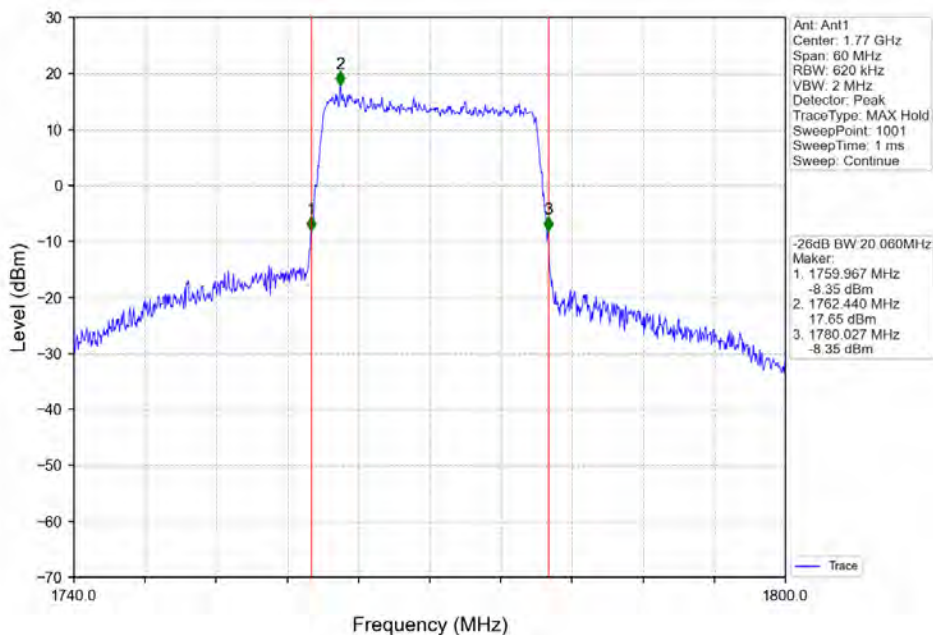
Band66_20MHz_64QAM_HCH_1770MHz_RB_100_0_NTNV
