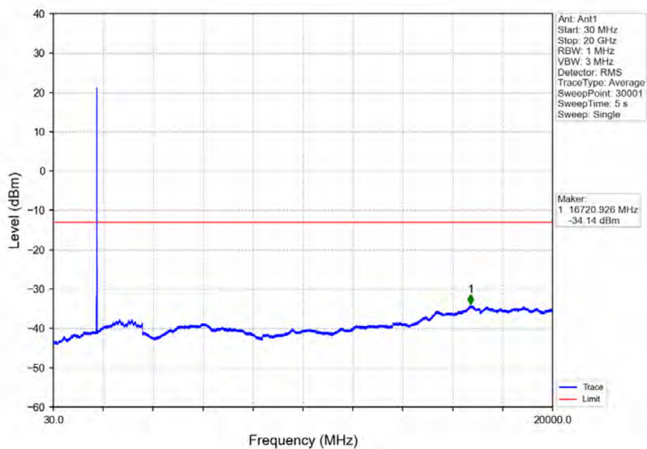
Band66_10MHz_64QAM_HCH_1775MHz_RB_1_49_NTNV
