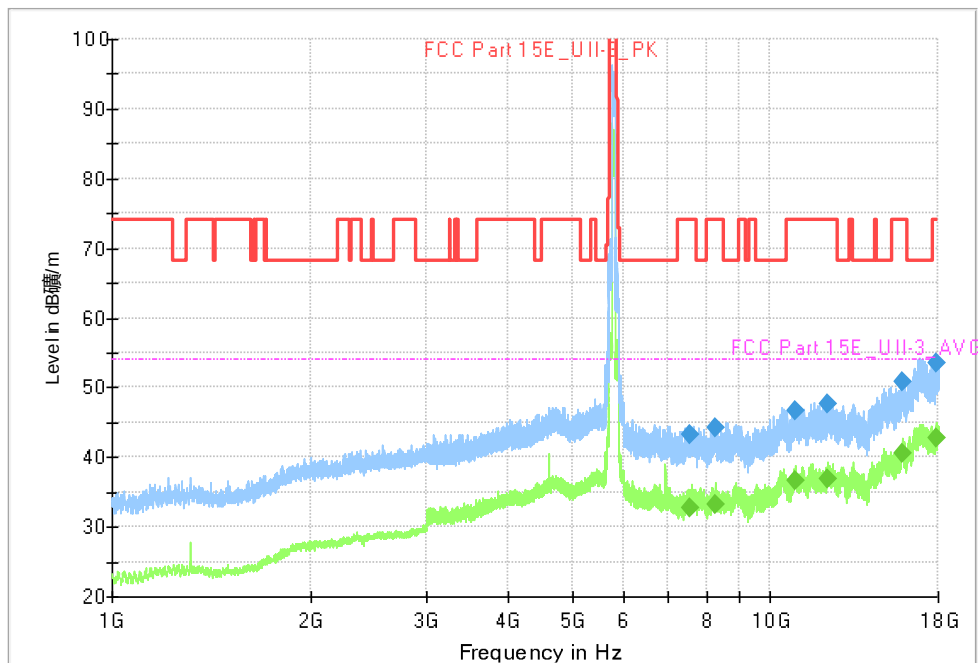
Fig. 92 Transmitter Spurious Emission (802.11ac-VHT80, CH155 5775MHz, 1 GHz ~18 GHz)
