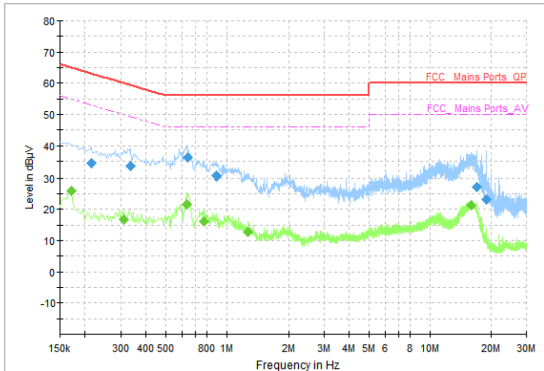
Fig. 97 AC Power line Conducted Emission (Traffic)
