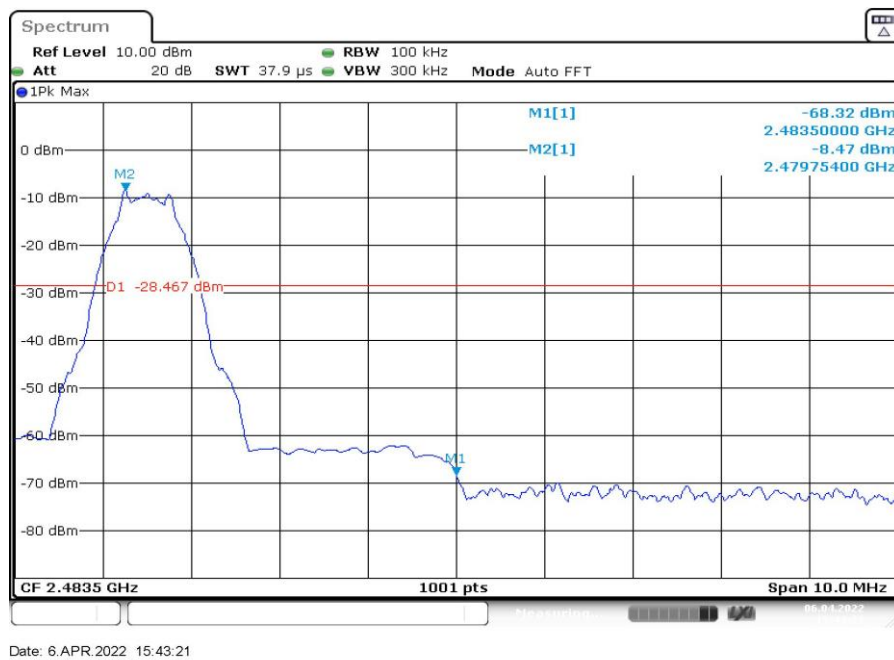
Fig.14 Band Edges (Ch 39), LE 1M
