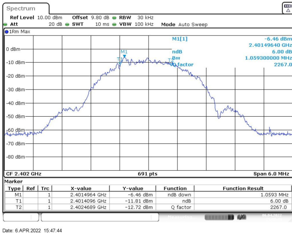
Fig.10 6dB Bandwidth (Ch 0), LE 2M
