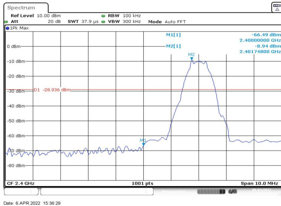
Fig.13 Band Edges (Ch 0), LE 1M
