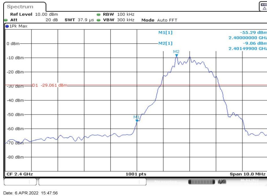
Fig.15 Band Edges (Ch 0), LE 2M
