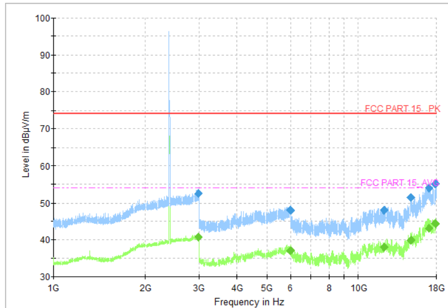
Fig.28 Radiated Spurious Emission (Ch0, 1 GHz ~18 GHz), LE 2M
