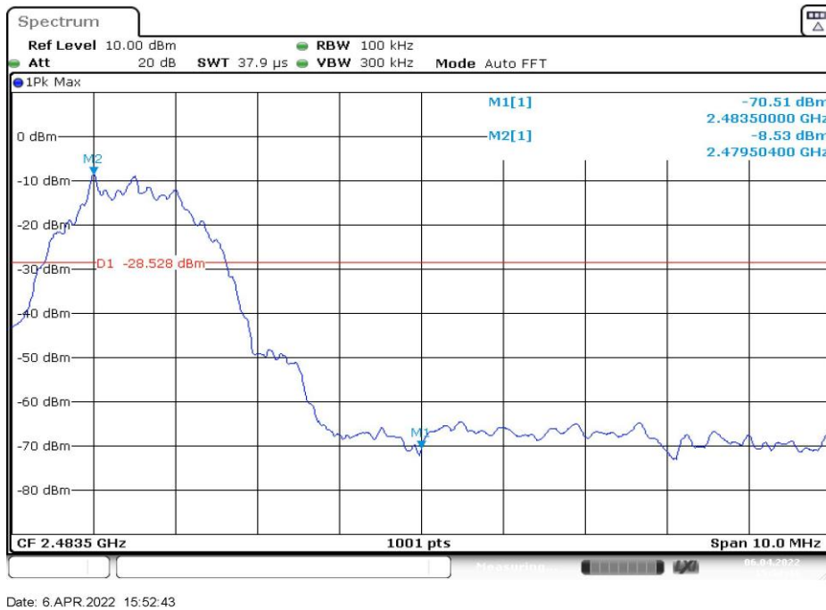
Fig.16 Band Edges (Ch 39), LE 2M
