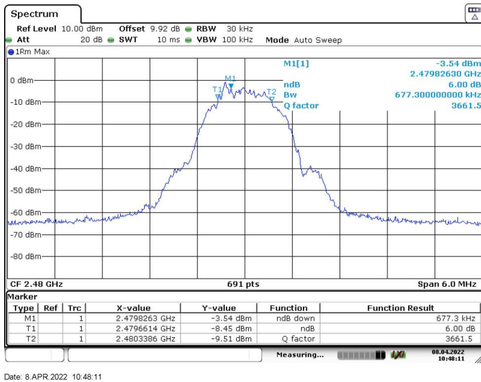
Fig.9 6dB Bandwidth (Ch 39), LE 1M
