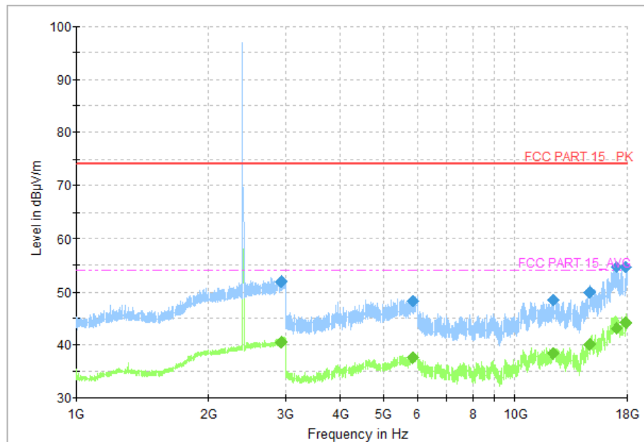
Fig.23 Radiated Spurious Emission (Ch0, 1 GHz ~18 GHz), LE 1M
