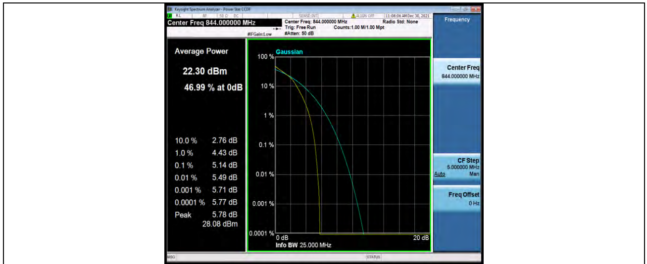
Band5-1.4MHz-64QAM-20407-1RB#0
